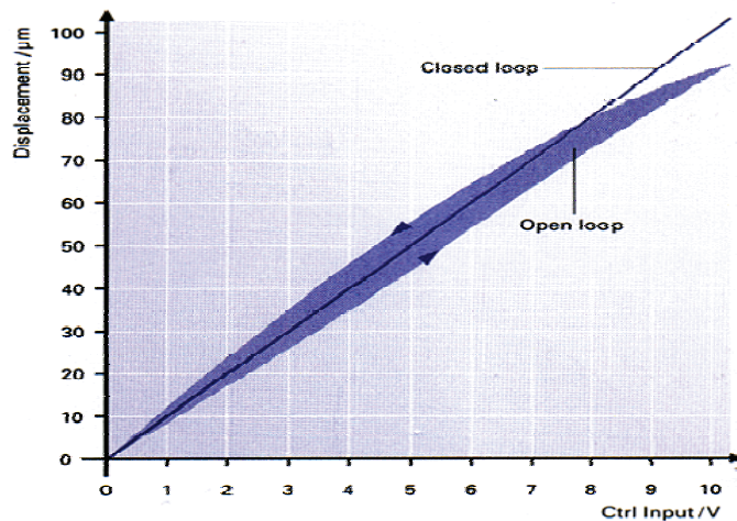
Fig. 2. Characteristic curve for PZT (from www.physikinstrumente.com )
