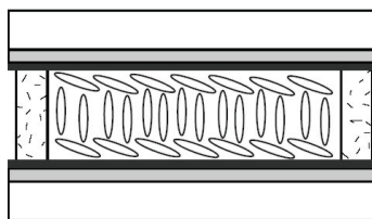
4.b: Minimal retardance V \gg 0
