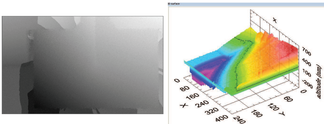
Fig.8. Unwrapped phase difference and displacement map between two loaded states for Compact Tension Notch Sample
