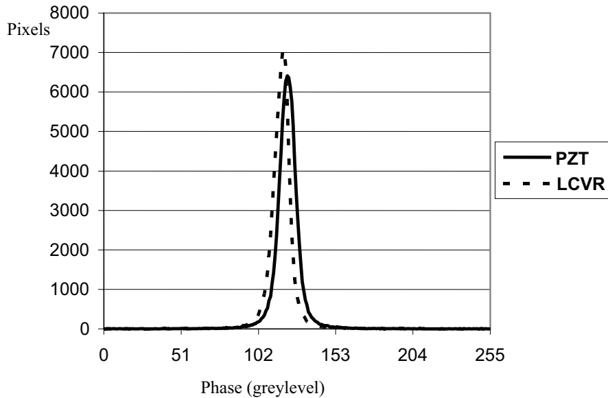
Fig.6. Histograms of the phase difference between two resting states (zero displacement)
