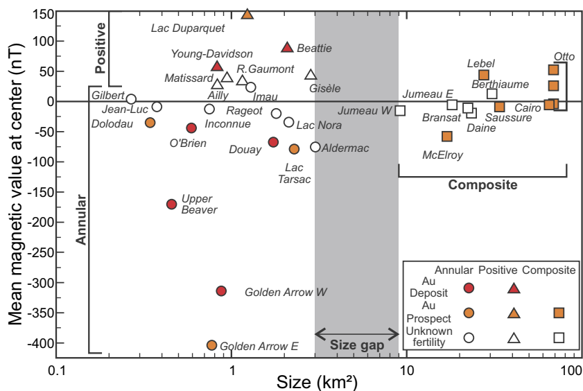
Fig. 7. Distribution of the three types of magnetic signatures vs. intrusion size and relationship to gold mineralization.
