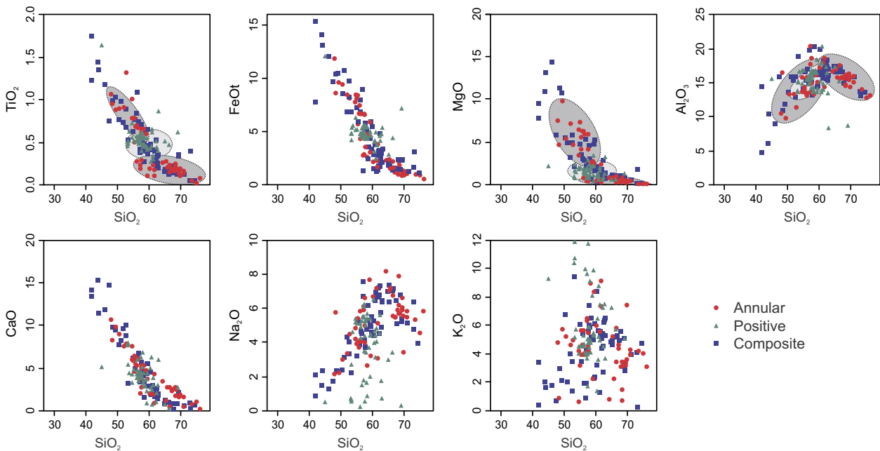
Fig. 6. Harker diagram showing almost linear evolutionary trends for \text{TiO}_2 , \text{MgO} , \text{FeO} , \text{CaO} , \text{Na}_2\text{O} and \text{Al}_2\text{O}_3 with differentiation ( \text{SiO}_2 increase) whereas \text{K}_2\text{O} has a more diffuse distribution.
