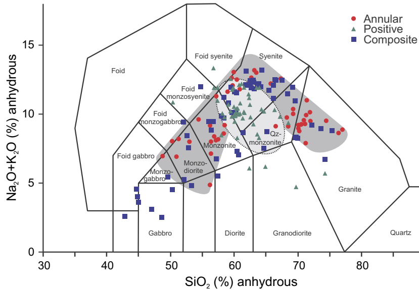
Fig. 5. Geochemistry of the intrusions highlighting alkali vs. silica-rich fields (Middlemost, 1985). The “positive” intrusions have homogeneous syenitic compositions, whereas “composite” and “annular” intrusions fall into both syenite to granite and more mafic monzonites to gabbro groups.
