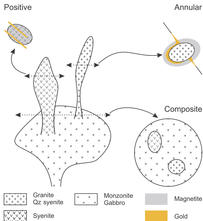
Fig. 8. The three intrusions type probable relationships and related gold settings.
