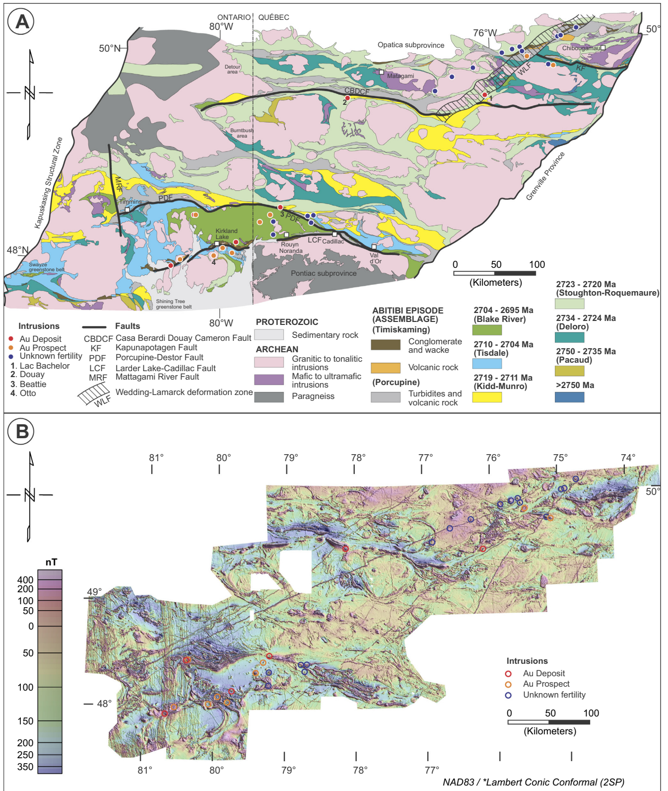
Fig. 1. (A) Location of the 31 alkaline intrusions studied on the Abitibi geology map (modified from Thurston et al., 2008 ). (B) Shaded residual total field Abitibi aeromagnetic image (derived from the GSC dataset described by Keating et al., 2010 ).
