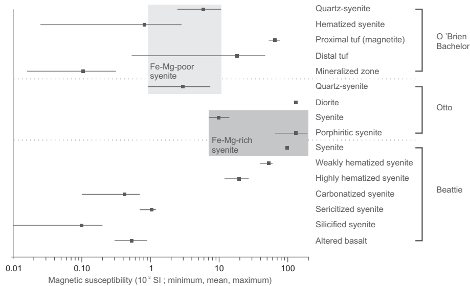
Fig. 3. Magnetic susceptibilities of the O'Brien, Otto and Beattie intrusions, related mineralized zones and host-rocks showing the correlation between lithology, alteration and magnetic susceptibility values.
