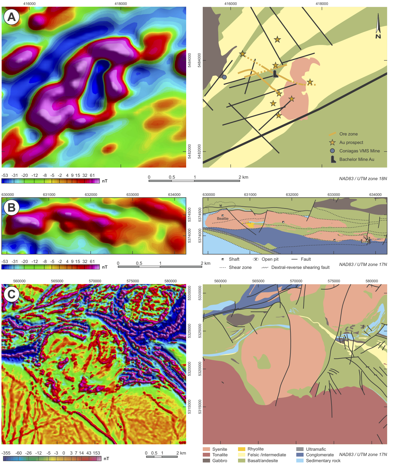
Fig. 2. Three magnetic signatures types. (A) "Annular", (B) "positive" – central magnetic high, (C) "composite" exemplified respectively by the O'Brien, Beattie and Otto intrusions.
