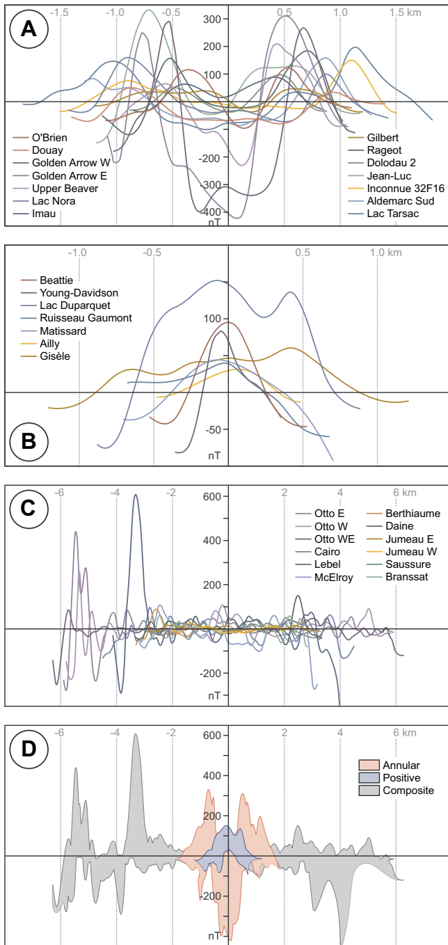
Fig. 4. Aeromagnetic profiles of the intrusions. (A) “Annular”, (B) “positive”, (C) “composite”, (D) synthesis of all three types.
