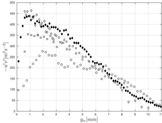
Figure 2: Impact of the spatial resolution of the PIV measurements on the accuracy of the Reynolds stresses . \diamond LDA measurements, \circ : Large Field of View (PIV), \square Intermediate Field of View (PIV), \blacklozenge Reduced Field of View (PIV)
