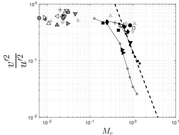
Figure 12: Ratio of normal stresses in subsonic and supersonic mixing layers. Symbols as in table 3. --- : 1/M_c^2 ; \blacktriangleright : present data ; \bullet : Langley consensus (Birch & Eggers (1973), Kline et al. (1980) ).
