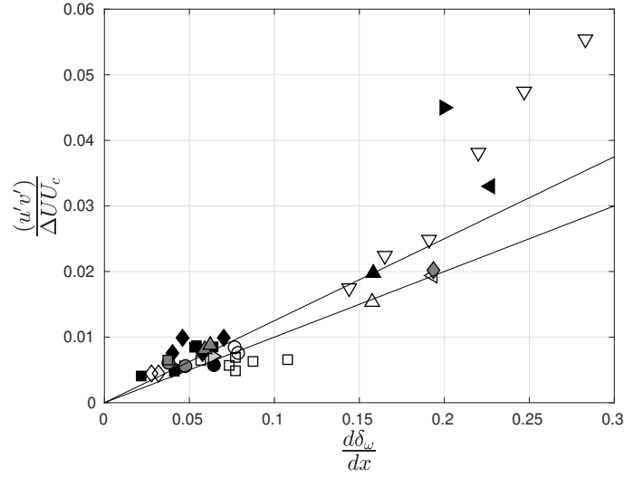
Figure 11: Relation between spreading rate and turbulent shear stress. Symbols as in table 3.
