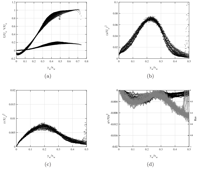
Figure 8: Velocity profiles in the wind tunnel coordinate system, \theta = 9.5^\circ : (a): longitudinal and normal velocity normalized by U_e ; (b): variance of the longitudinal velocity; (c): variance of the normal velocity; (d): cross correlation (black lines) and correlation coefficient (gray lines, right axis).
