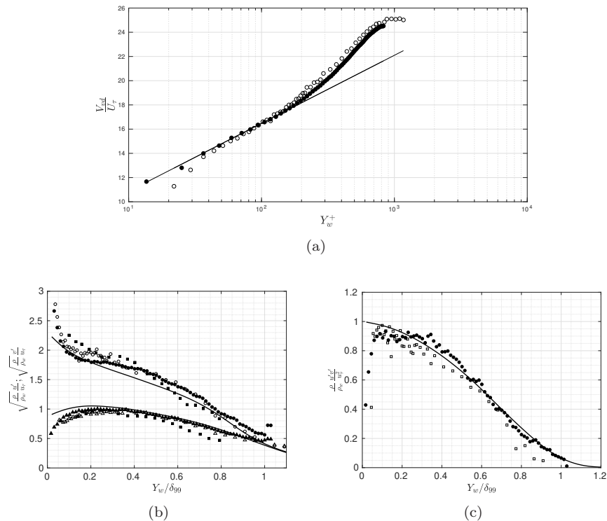
Figure 3: Comparison LDA vs PIV velocity measurements in the upstream boundary layer. Closed symbols PIV (reduced FOV); open symbols LDA. (a): mean velocity in Van Driest representation. (b): Longitudinal ( \circ ) and normal ( \triangle ) R.m.s. velocity in Morkovin representation ( \blacksquare Humble et al. (2009a)). (c): Reynolds shear stress in Morkovin representation. Black lines: Klebanoff's data (M=0, Klebanoff (1954)).
