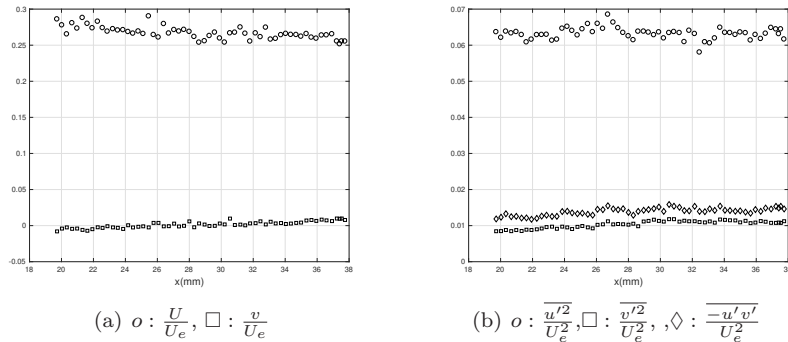
Figure 6: Evolution along the estimated centerline of the mean longitudinal and vertical velocity (a) and of the Reynolds stresses (b) in the mixing layer coordinate system and for \theta = 9.5^\circ .
