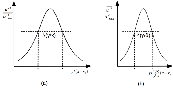
Figure 10: Method for determination of the spreading rate
