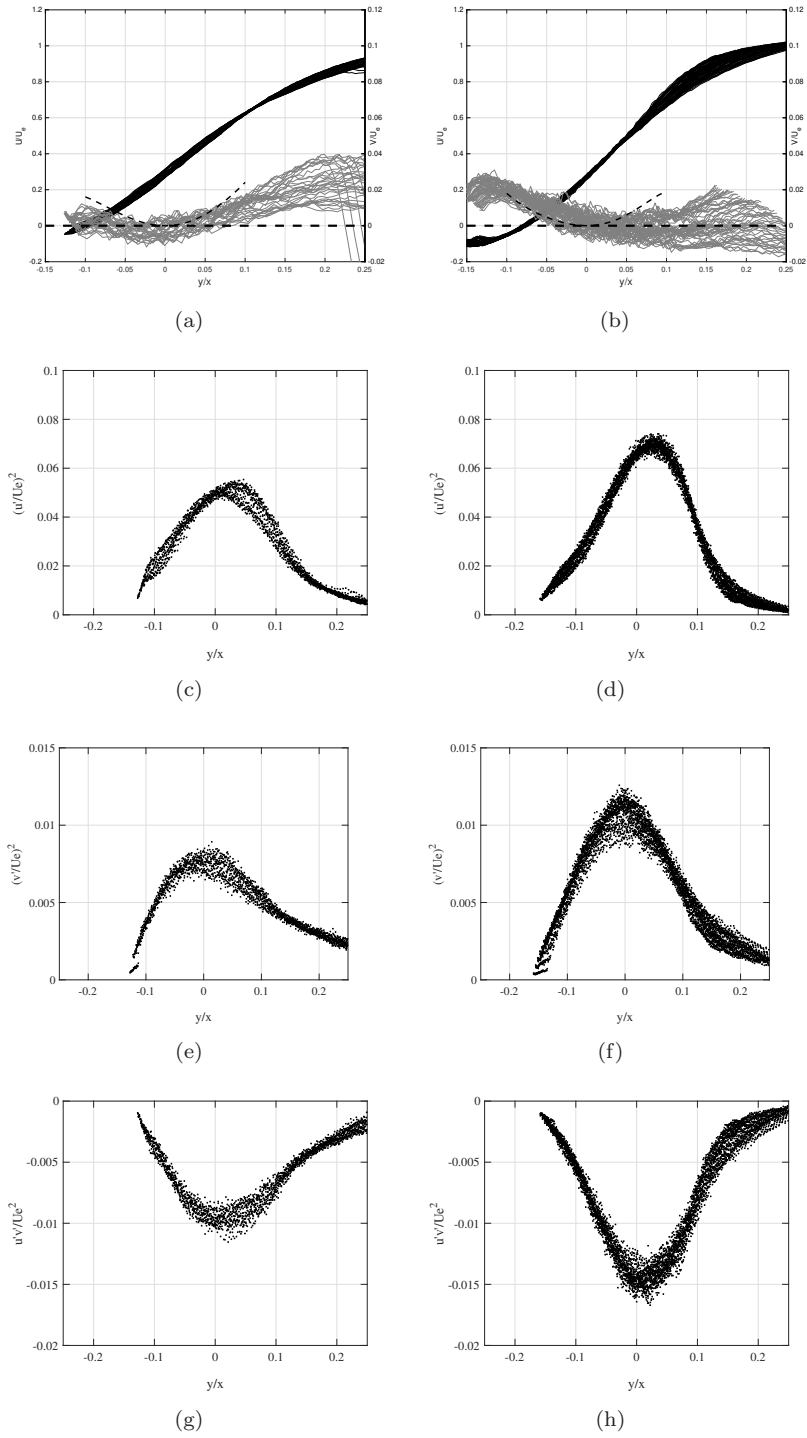
Figure 7: Velocity profiles in the mixing layer coordinate system, \theta = 8^\circ (left column) and \theta = 9.5^\circ (right column). (a), (b): black dots: mean longitudinal velocity normalised by U_e , grayline V/U_e , dashed line V/U_e determined from conservation; (c),(d): variance of the longitudinal velocity; (e), (f): variance of the normal velocity; (g), (h): turbulent shear stress. All stresses normalised by U_e^2 .
