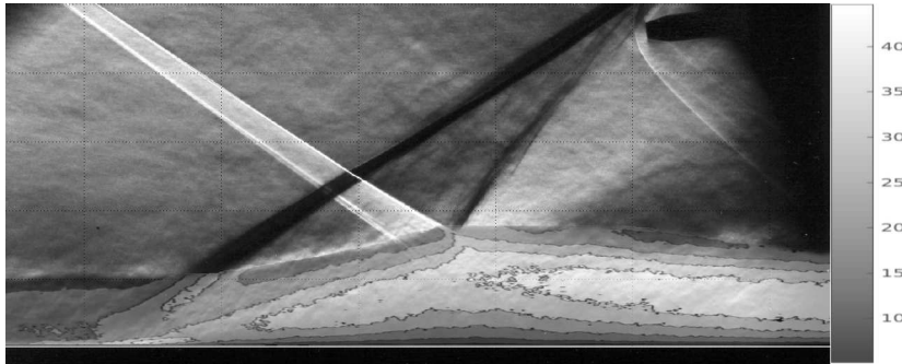
Figure 1: Spark schlieren visualisation of the interaction, for a deflection angle of 9.5^\circ . Superimposed to the Schlieren visualisation, the standard deviation of the vertical velocity component in the frame of reference of the wind tunnel, obtained by PIV measurements (grey scale associated, [m.s^{-1}] ).
