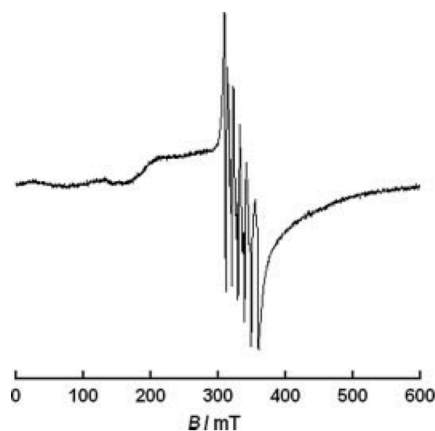
Figure 5. X-band EPR spectra of 1 (PF 6 ) 2 ( 10^{-3} M in 50 mM aqueous PIPES buffer, pH 7.5). Microwave frequency: 9.38 GHz; microwave power: 2.0 mW; modulation amplitude: 0.5 mT; modulation frequency: 100 kHz; gain: 20 dB.
