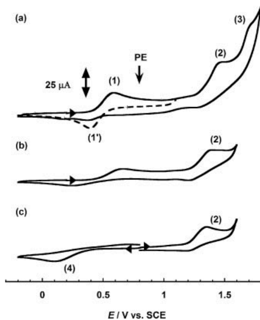
Figure 3. Cyclic voltammograms of 1(\text{PF}_6)_2 (1.1 mM in \text{CH}_3\text{CN} with 0.1 M tetrabutylammonium perchlorate) under argon ( \nu = 0.1 \text{Vs}^{-1} ; working electrode: glassy carbon; counter electrode: Pt wire; reference electrode: \text{Ag}/\text{AgClO}_4 ) at 20 (a) -25 (b), and -25 °C after electrolysis at E = +0.8 V vs. SCE (c). PE = potential of the preparative electrolysis.
