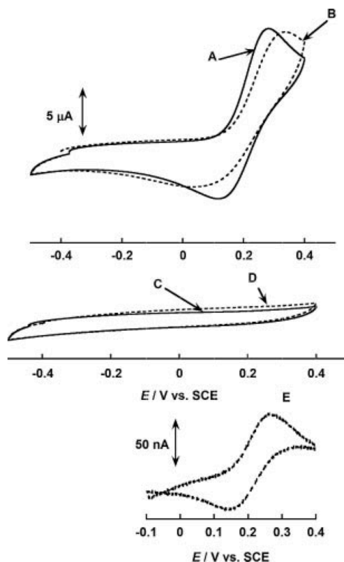
Figure 6. Cyclic voltammograms in aqueous solution: (A) 1 (PF 6 ) 2 ( 10^{-3} M) in aqueous PIPES buffer (pH 7.5, 50 mM) and (B) in aqueous phosphate buffer (pH 7.8, 50 mM); (C) MnCl_2 ( 10^{-3} M) in aqueous PIPES buffer (pH 7.5, 50 mM) and (D) in aqueous phosphate buffer (pH 7.8, 50 mM); (E) 1 (PF 6 ) 2 ( 10^{-5} M) in aqueous PIPES buffer (pH 7.5, 50 mM); the signal recorded for pure PIPES buffer has been subtracted. Working electrode: glassy carbon; counter electrode: Pt wire; reference electrode: SCE.
