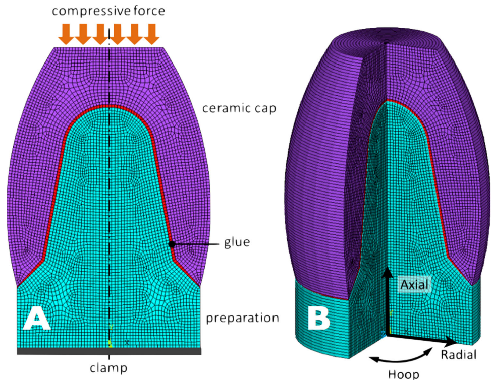
Fig. 2 FE model for the ceramic restoration with the PI design. The model takes into account three components: the preparation, the ceramic cap and the glue. a Sagittal cut. Red arrows indicate the orientation of the compressive force. b Expanded volume (3/4 expansion). Black arrows indicate the direction of the exerted stresses
