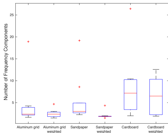
Figure 8: Box-whisker plot of the experimental results. The data show the discrimination threshold for the number of frequency components needed so that the original and the reproduced signal were still discriminable. ANOVA analysis showed that the texture type was significant for the number of frequency components. However, the type of the method (weighted or unweighted) had no significant influence.
