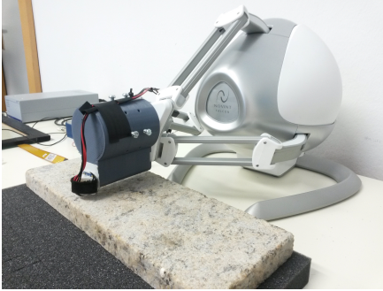
Figure 2: The data recording system. An accelerometer on a tool tip that is mounted on the force feedback device scans surfaces horizontally with a constant velocity of 80 mm/s.
