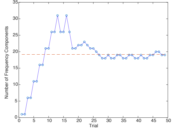
Figure 7: An example data set collected by one up-two down adaptive staircase method. The x-axis shows the number of trials and the y-axis shows the number of frequency components from which the texture signal is reproduced. When the user can distinguish original and reproduced signal, further frequency components are added to the reproduced signal.
