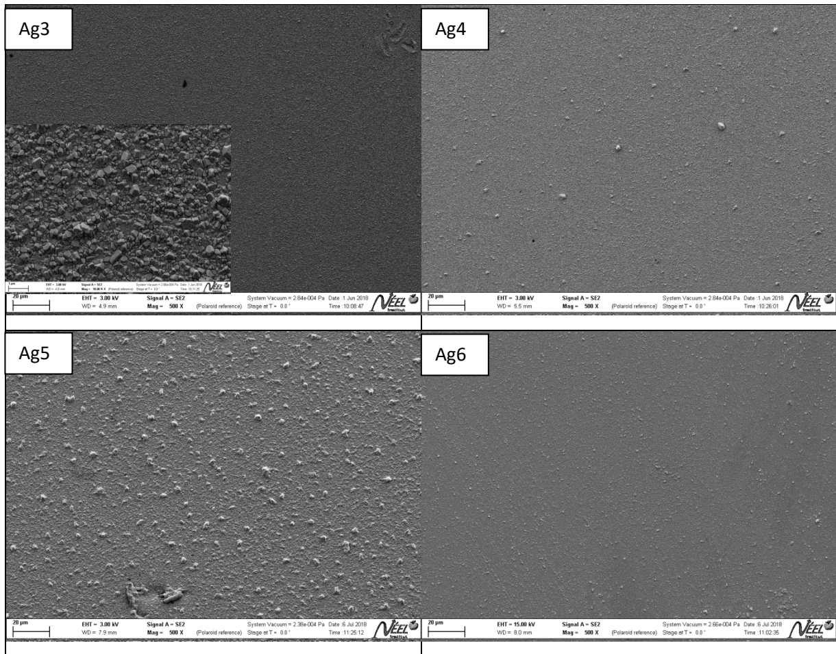
Figure 4 : SEM images of the Ag1-Ag6 films prepared under different conditions process.
