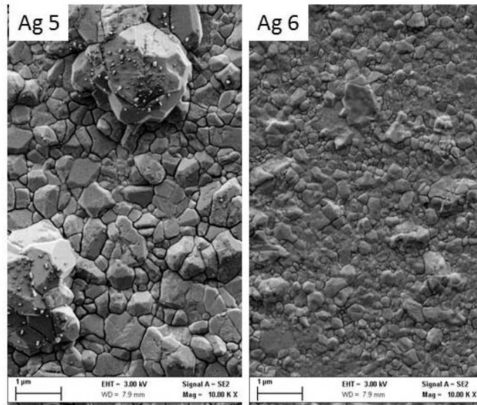
Figure 8 : SEM images of the Ag5 and Ag6 films at x10000 magnification.
