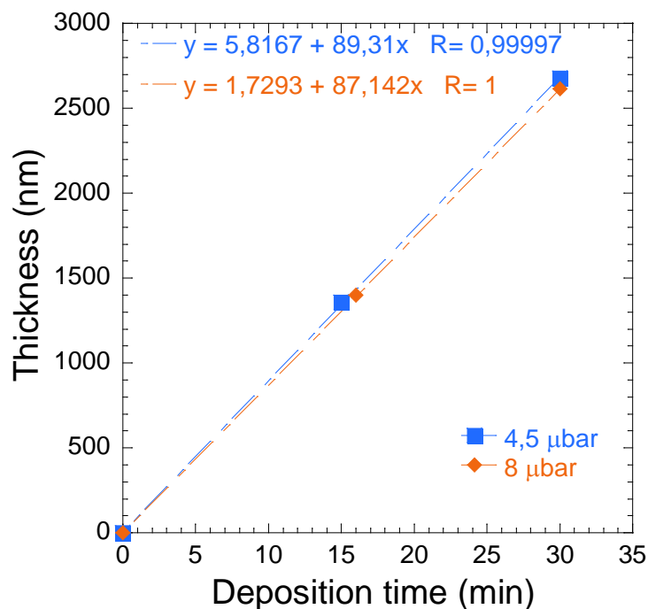
Figure 1 : Thickness versus deposition time for a argon pressure of 4,5 and 8 \mu bar.
