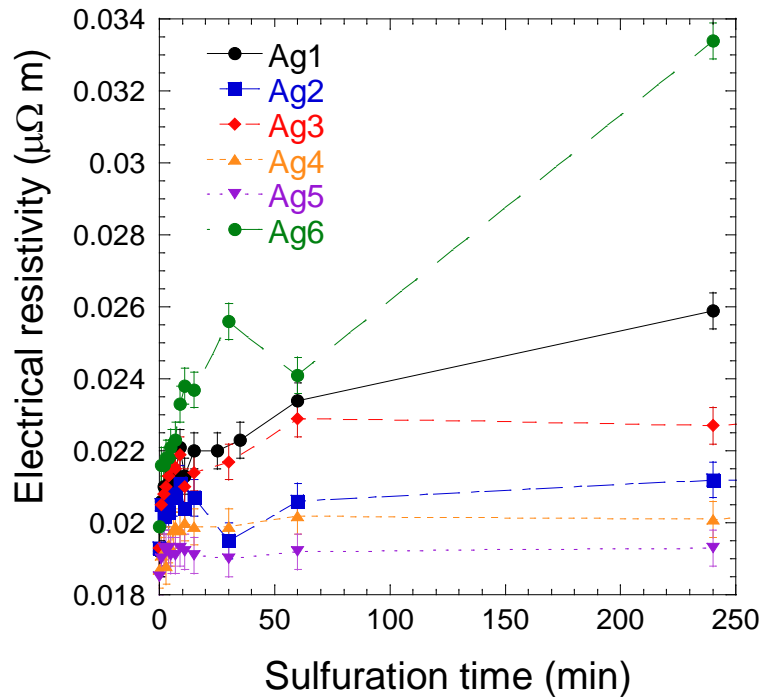
Figure 6: Long sulfurization time dependence of the electrical resistivity for Ag films deposited under different conditions (Ag1-Ag6).
