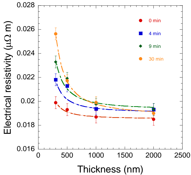
Figure 7: Electrical resistivity versus film thickness for different sulfurization times.
