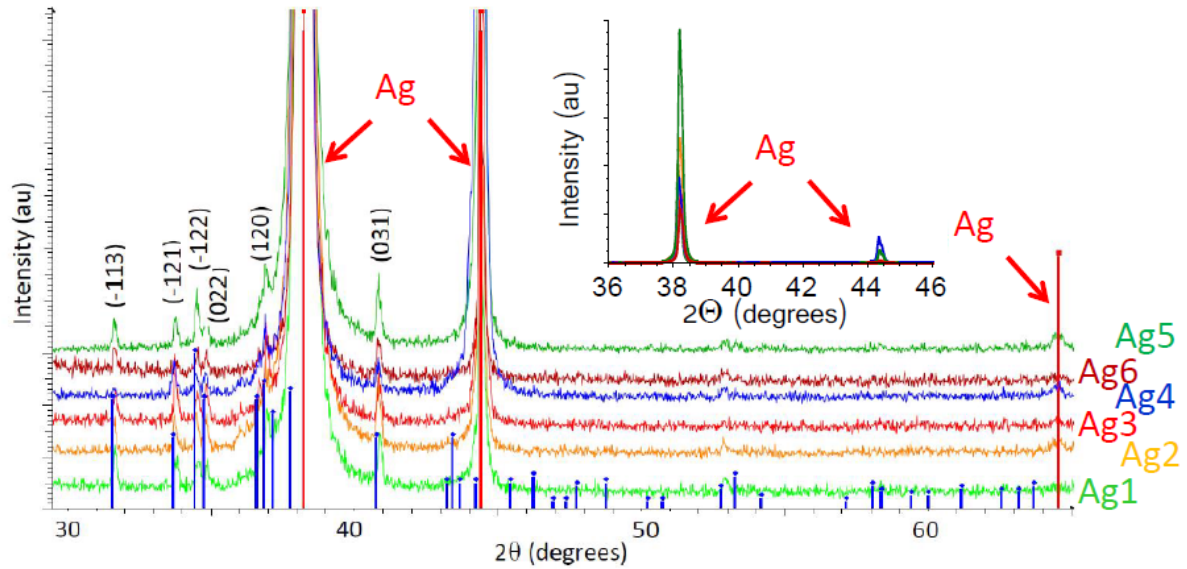
Figure 3: X-ray diffraction patterns of Ag films deposited under different conditions after a sulfurization time of 120 min. Peaks of the Ag (in red, JCPDS Card File: 00-087-0718) and \alpha - \text{Ag}_2\text{S} (acanthite) (in blue, JCPDS Card File: 00-014-0072) are marked.
