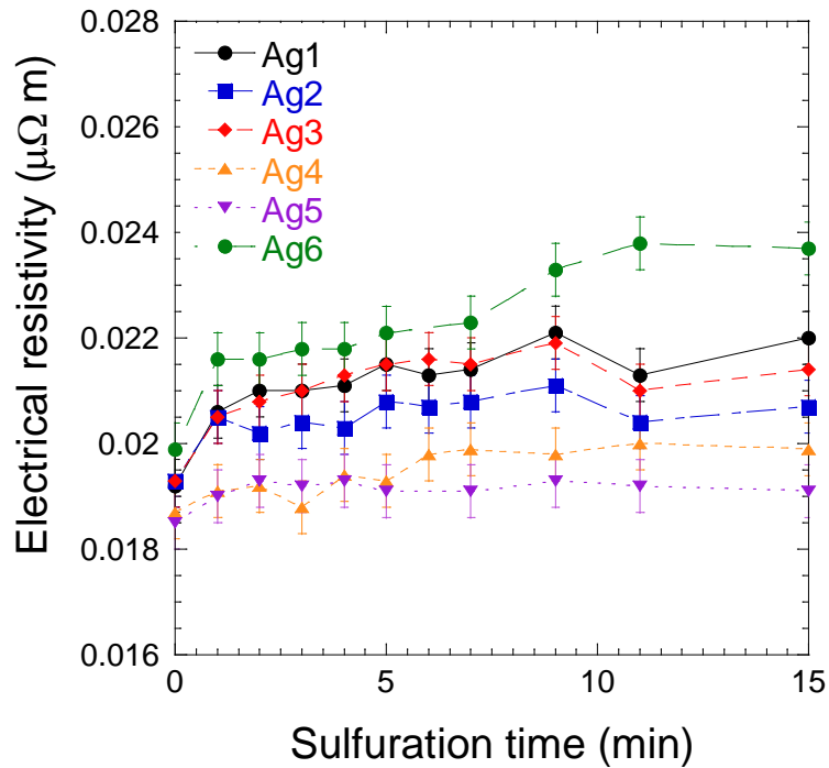
Figure 5: Electrical resistivity versus sulfuration time for Ag films deposited under different conditions (Ag1-Ag6).
