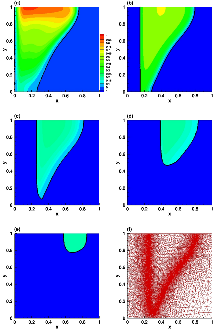
Figure 11: Solidification of the PCM after a partial melting. Temperature iso-lines in the fluid phase. The solid part is represented in blue and corresponds to the region of temperature \theta \leq \theta_f = 0 . Time instants (panels a to e): t_\varphi = 59 min, t_\varphi = 70 min, t_\varphi = 90 min, t_\varphi = 131 min and t_\varphi = 200 min. The adapted mesh corresponding to t_\varphi = 90 min is plotted in panel (f). r_\delta \times \mathcal{Ra} = 3.27 \cdot 10^5 .
