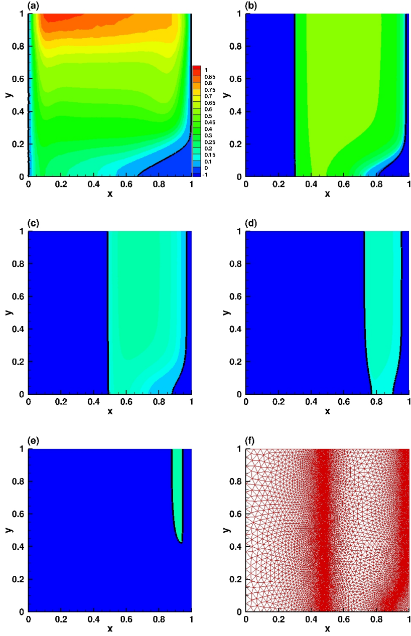
Figure 10: Solidification of the PCM after a complete melting. Temperature iso-lines in the fluid phase. The solid part is represented in blue and corresponds to the region of temperature \theta \leq \theta_f = 0 . Time instants (panels a to e): t_\varphi = 185 min, t_\varphi = 231 min, t_\varphi = 300 min, t_\varphi = 430 min and t_\varphi = 510 min. The adapted mesh corresponding to t_\varphi = 300 min is plotted in panel (f). r_\delta \times Ra = 3.27 \cdot 10^5 .
