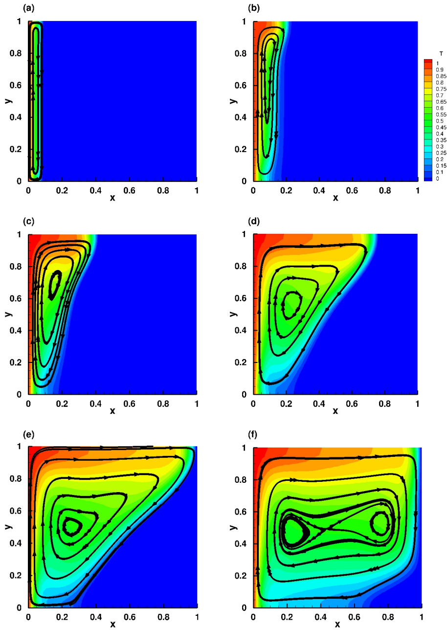
Figure 5: Complete melting of the PCM. Temperature iso-lines and streamlines in the fluid phase. The solid part is represented in blue and corresponds to the region of temperature \theta \leq \theta_f = 0 . Time instants (panels a to f): \tau = 0.004; 0.016; 0.032; 0.063; 0.08; 0.2 . Ra = 3.27 \cdot 10^5 , Pr = 56.2 and Ste = 0.045 .
