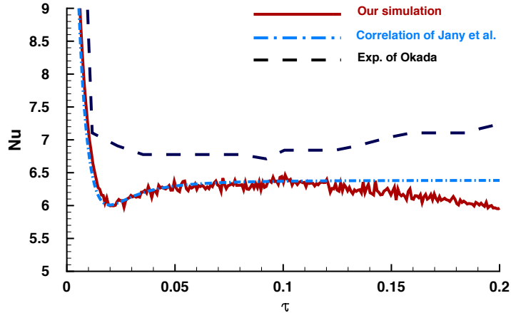
Figure 6: Complete melting of the PCM. Time evolution of the average Nusselt number defined at the hot (left) wall (cf. eq. 21) (solid line). Comparison with the experimental results of Okada (1984) (dashed line) and the predictions using the correlation (22) suggested by Jany and Bejan (1988) (dash-dot line). \mathcal{Ra} = 3.27 \cdot 10^5 , \text{Pr} = 56.2 and \mathcal{Ste} = 0.045 .
