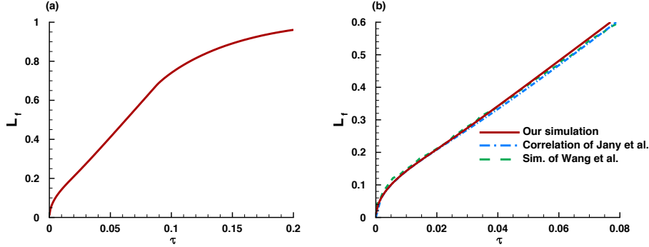
Figure 7: Complete melting of the PCM. (a) Time evolution of the liquid fraction for the complete melting of the PCM. (b) Comparison of our results (solid line) with the numerical results of Wang et al. (2010a) (dashed line) and the predictions using the correlation (23) suggested by Jany and Bejan (1988) (dash-dot line).
