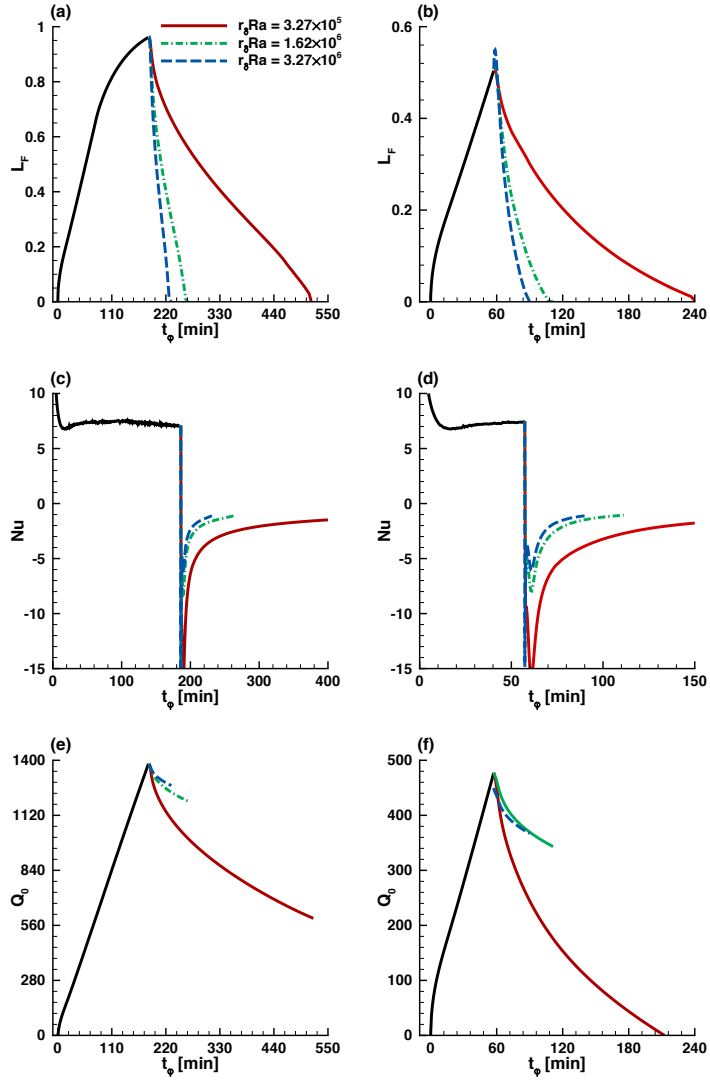
Figure 12: Temporal evolution of the liquid fraction ( L_f ), the Nusselt number Nu , and the accumulated heat input Q_0 during the entire melting-solidification cycle. Case CM, (left); Case PM, (right).
