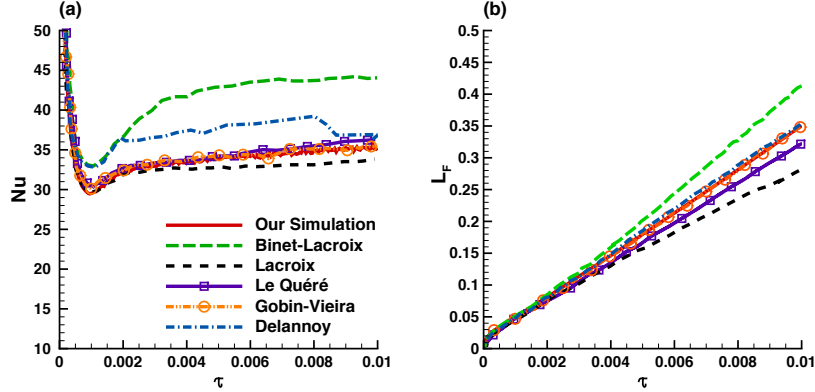
Figure 4: Time evolution of the Nusselt number (a) and the liquid fraction (b) compared with five simulations presented by Bertrand et al. (1999). \mathcal{Ra} = 2 \cdot 10^8 , \text{Pr} = 50 and Ste = 0.1 .
