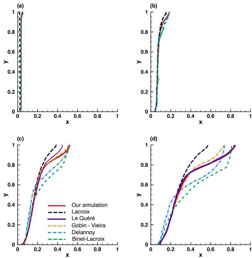
Figure 3: Location of the solid-liquid interface at dimensionless time (panels a to d) \tau = 0.0005 , \tau = 0.002 , \tau = 0.006 and \tau = 0.01 , compared with five simulations presented by Bertrand et al. (1999). Ra = 2 \cdot 10^8 , Pr = 50 and Ste = 0.1 .
