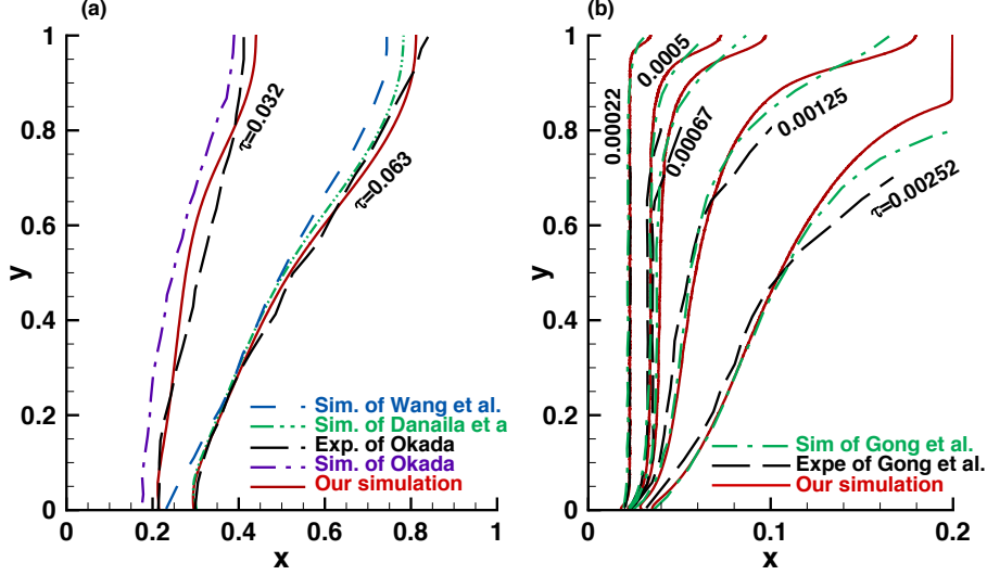
Figure 2: Location of the interface during the melting of the PCM. (a) Comparison with experimental data of Okada (1984) and numerical results of Danaila et al. (2014) and Wang et al. (2010a) for two time instants ( \tau = 0.032 and 0.063 ). \mathcal{Ra} = 3.27 \cdot 10^5 , \text{Pr} = 56.2 and \text{Ste} = 0.045 (b) Comparison with both experiment and simulation of Gong et al. (2015) for five time instants ( \tau = 0.0002, 0.00050, 0.00067, 0.00125, 0.00252 ). \mathcal{Ra} = 2.48 \cdot 10^8 , \text{Pr} = 50 and \text{Ste} = 0.072 .
