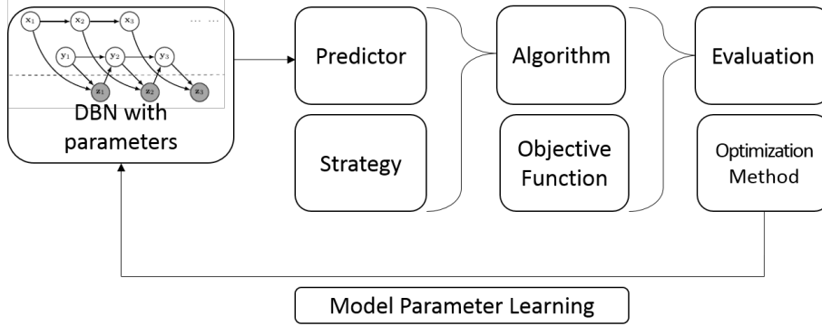
FIG 4. Learning process for our DBN. Once an architecture has been decided, we combine this with a strategy to create an systematic algorithm. We select an objective function that provides an Evaluation function. We use an optimization method to find the best parameters according to our evaluation function. We monitor overall performance of the trading strategy on a separate test set to validate scarce overfitting.
