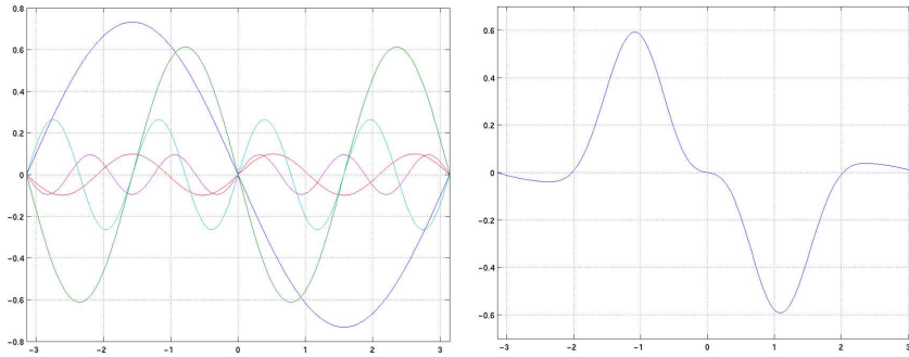
Fig. 4. Function V_c(\theta) used for 2D control, obtained by smoothing profile from Clustering Genetic Algorithm.
