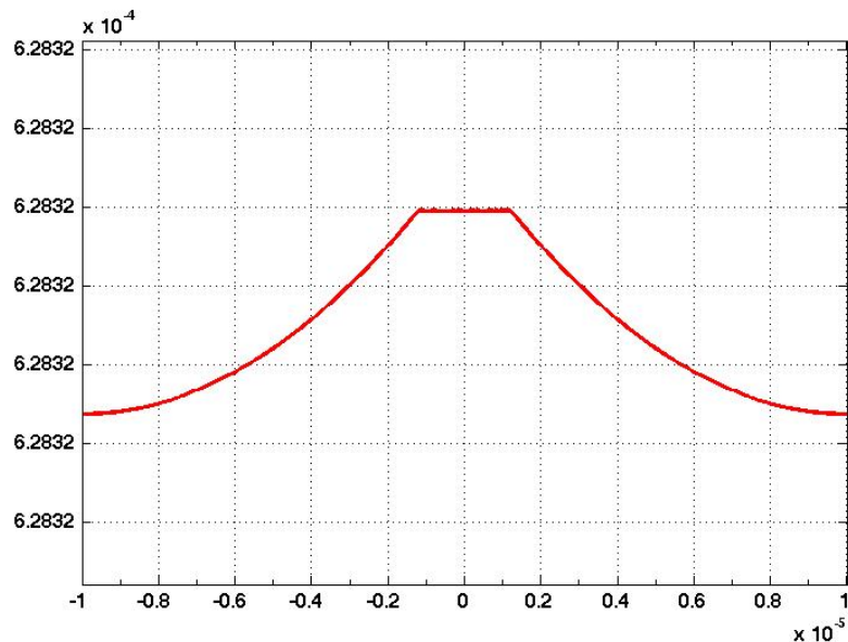
Figure 6: Solution u(x, t) to the equation (10) at t = 0.1 with \delta t = 10^{-4} .
