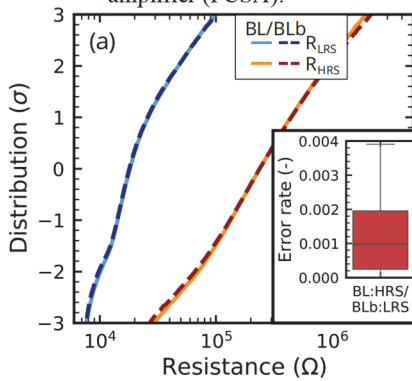
Fig. 6. (a) Distribution of resistance for bit '1' (BL:HRS/BLb:LRS) and bit '0' (BL:LRS/BLb:HRS) in the case of a checkerboard type of programming the memory array. (b-c) Failure rate on 100 programming according differential sense for two checkerboards configuration. V_{appReset}=2.5V , t_{pulse}=1\mu s , I_c=55\mu A .
