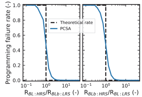
Fig. 7. Rate of programming failure indicated by the PCSA circuit as function of R_{HRS}/R_{LRS} ratio obtained by a high-resolution resistance measurement @ V_{read} = 0.1V .
