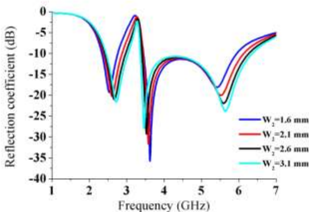
Figure. 8. Reflection coefficient S_{11} for various values of W_2 .
