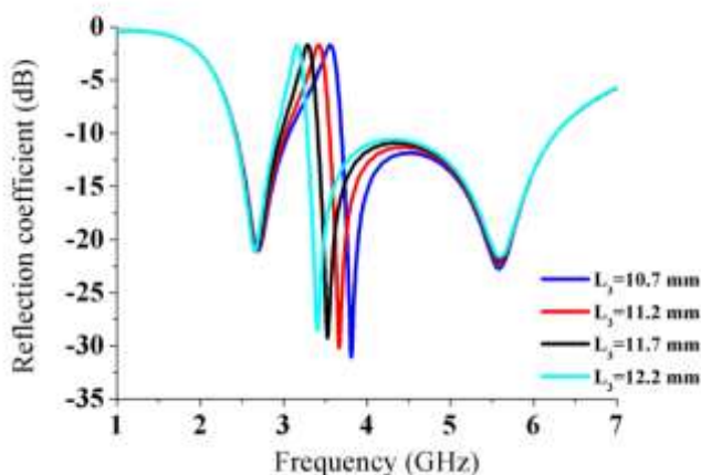
Figure. 7. Reflection coefficient S_{11} for various values of L_3 .
