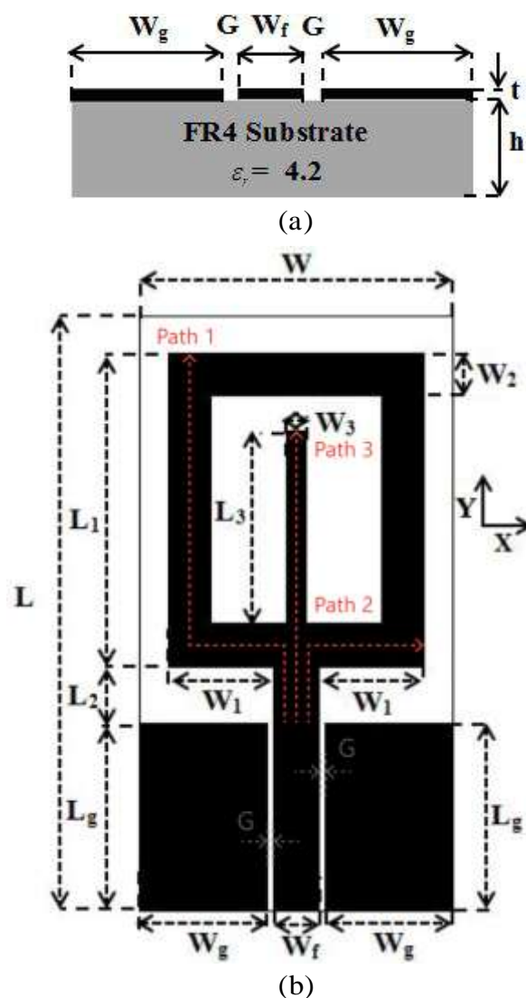
Figure. 1. Geometry of the proposed antenna: (a) side view, (b) top view.
