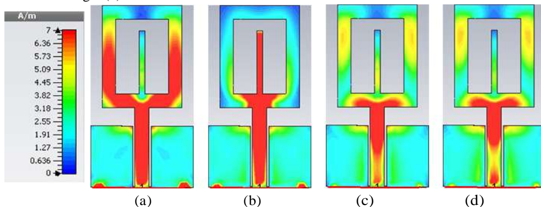
Figure. 11. Simulated surface current distributions of the proposed antenna at (a) 2.60 GHz, (b) 3.50 GHz, (c) 5.20 GHz and (d) 5.50 GHz.
