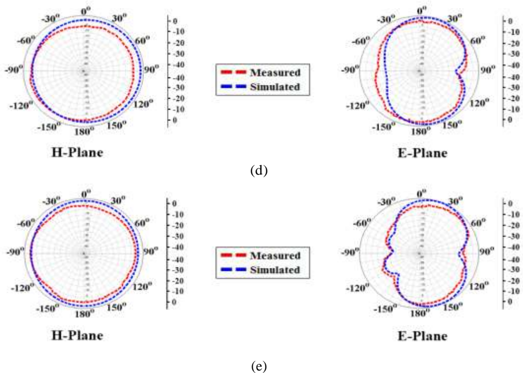
Figure. 12. Comparison between simulated and measured radiation patterns of the proposed antenna at frequencies (a) 2.40 GHz, (b) 2.60 GHz, (c) 3.50 GHz, (d) 5.20 GHz and (e) 5.50 GHz.
