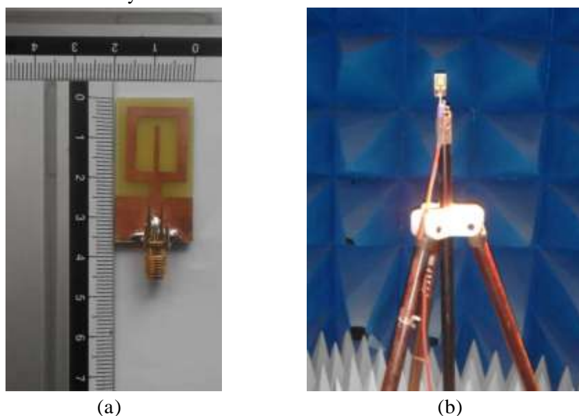
Figure. 9. (a) Fabricated prototype antenna, (b) proposed antenna in anechoic chamber.
