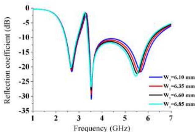
Figure. 5. Reflection coefficient S_{11} for various values of W_1 .
