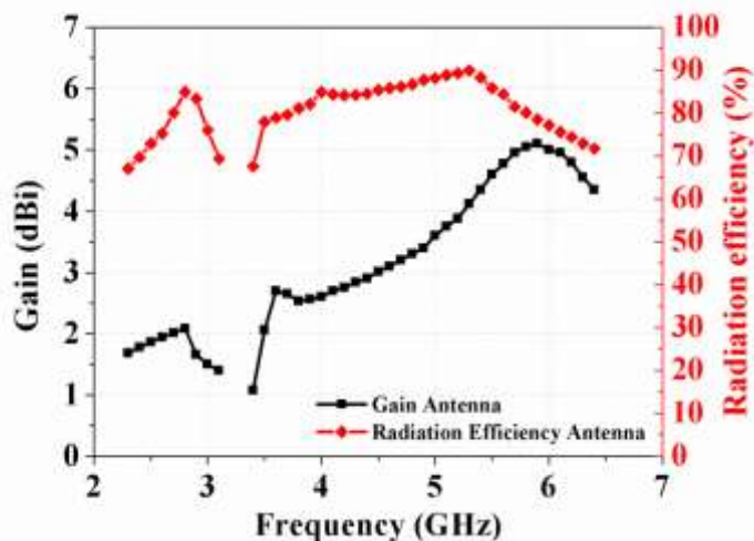
Figure. 13. Simulated gain and radiation efficiency with respect to frequency for the proposed antenna.
