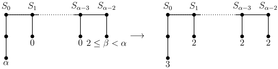
(b) Case 3, 2 \leq \beta < \alpha
