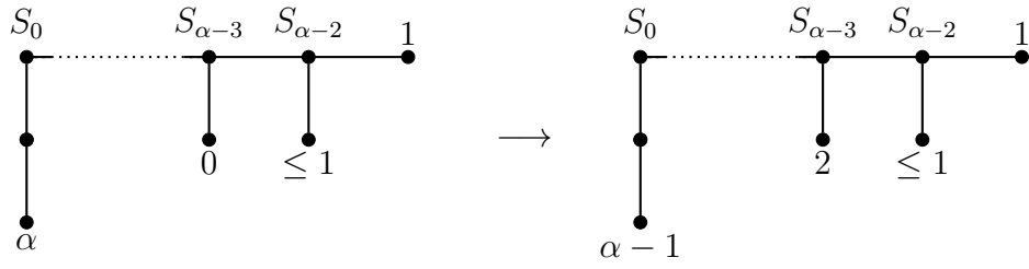
(a) Case 1, S_{\alpha-2} is of type \mathcal{S}_1
