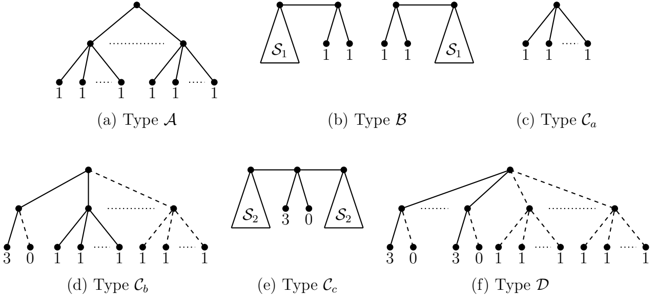
Figure 2: Spine-subtrees of given special types.
