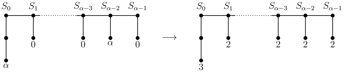
(c) Case 3, \beta = \alpha and \ell_{\alpha-1} is f -dominated only by \ell_{\alpha-2}
