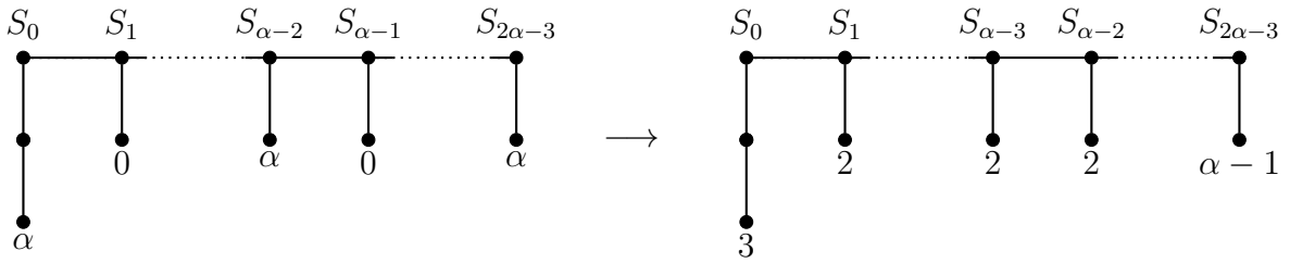
(d) Case 3, \beta = \alpha and \ell_{\alpha-1} is f -dominated by \ell_{\alpha-2} and x = \ell_{2\alpha-3}
