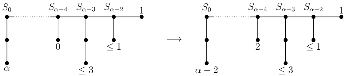
(b) Case 1, S_{\alpha-2} is of type \mathcal{S}_2
