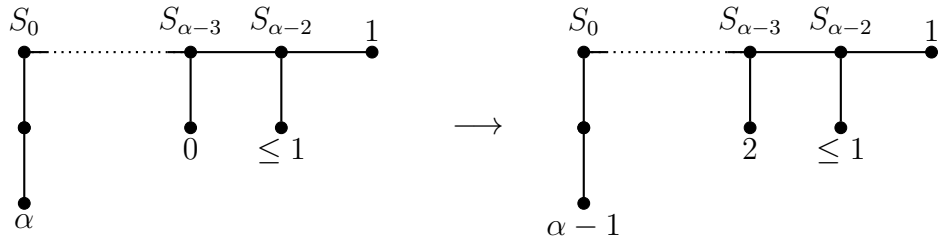
(a) Case 1, S_{\alpha-2} is of type \mathcal{S}_1
