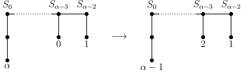
(a) Case 3, \beta = 1
