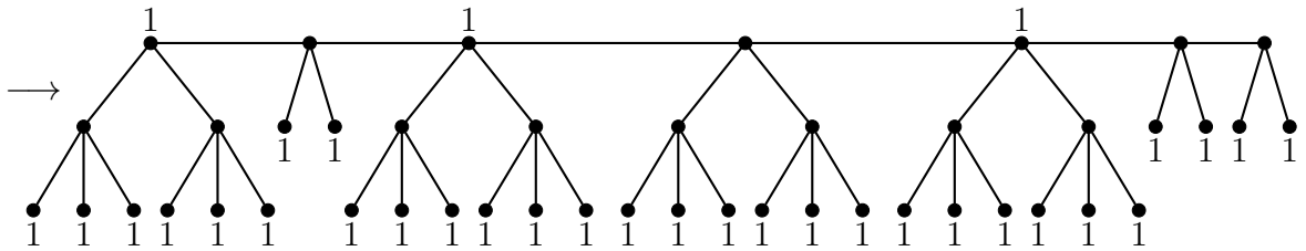
(d) From f_3 to f_4 , for a sequence of type \langle \emptyset \rangle \mathcal{A} \mathcal{C}_c \mathcal{A} \mathcal{A} \mathcal{A} \langle \mathcal{B} \mathcal{B} \rangle (cost increases by 2)
