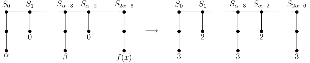
(b) Case 4(b), \beta \geq 7 , \beta - 1 \leq f(x) \leq \beta and \ell_{\alpha-2} is f -dominated by \ell_{\alpha-3} and x = \ell_{2\alpha-6}
