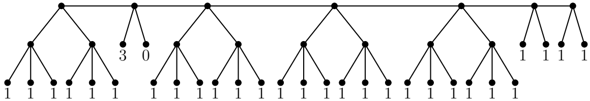
(c) From f_2 to f_3
