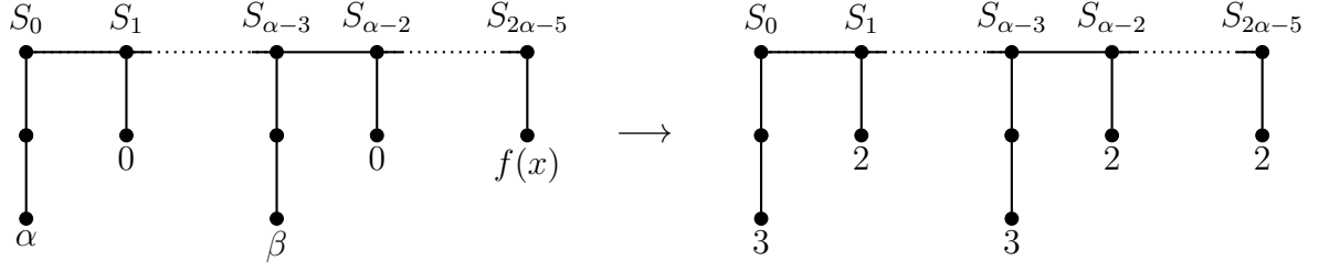
(a) Case 4(a), \beta \geq 7 , \beta - 1 \leq f(x) \leq \beta and \ell_{\alpha-2} is f -dominated by \ell_{\alpha-3} and x = \ell_{2\alpha-5}
