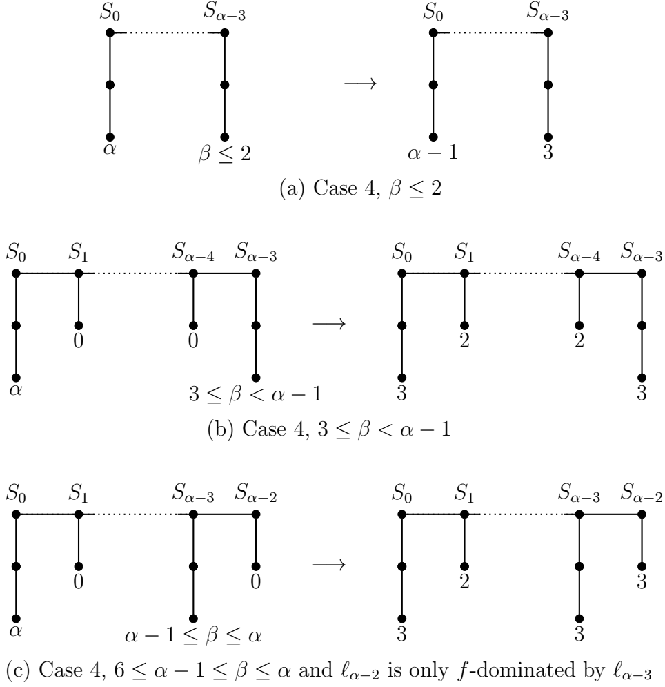
Figure 6: Independent broadcasts for the proof of Lemma 24, case 4 (only one branch per spine-subtree is depicted).
