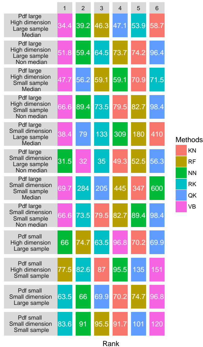
Figure 15: Summary of the rank and the error of the methods. The methods are ranked with respect to the expectation of their rank on the associated class of problems. The expectation of E_{CQ} is provided in white at the center of the cell.
