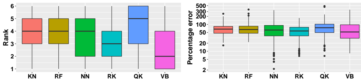
Figure 8: Boxplots of ranks and E_{CQ} error over the entire benchmark. Note that for clarity, the right boxplots do not contain the error of the median for the toy problem 2.
