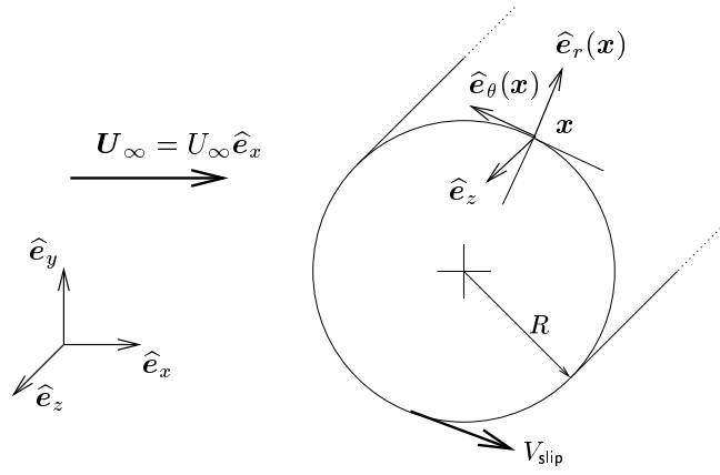
FIGURE 1. Cartesian and cylindrical basis.
