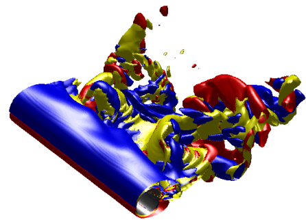
Fig. 12 : Effect of 3D control of 3D flow at large energies and large wavelength (locked on mode A).
