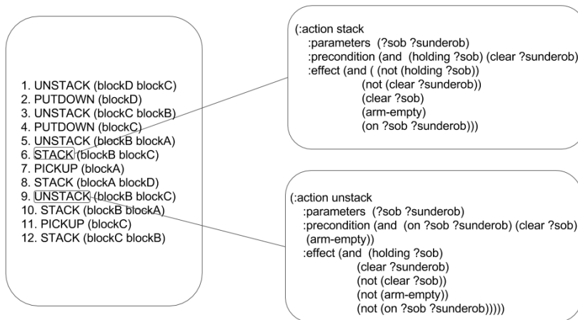
Figure 4: PDDL Representation Of the actions stack and unstack in the Blocksworld domain
