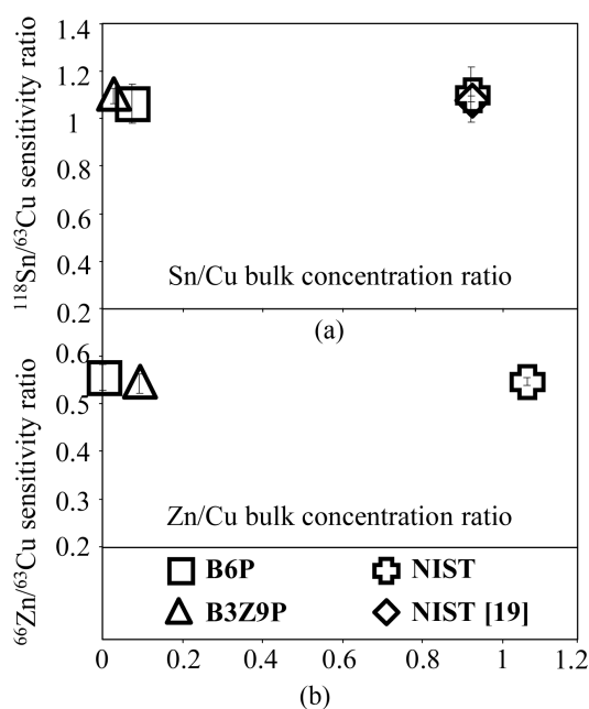
Figure 2. (a) Sn/Cu average sensitivity ratios vs. Sn/Cu bulk concentration ratio for alloys (B6P and B3Z9P) and NIST-SRM-610 reference materials. For comparison, also shown are the values obtained previously [19] for NIST-SRM-610; (b) Zn/Cu average sensitivity ratios vs. Zn/Cu bulk concentration ratio for alloys (B6P and B3Z9P) and NIST-SRM-610 reference materials.
