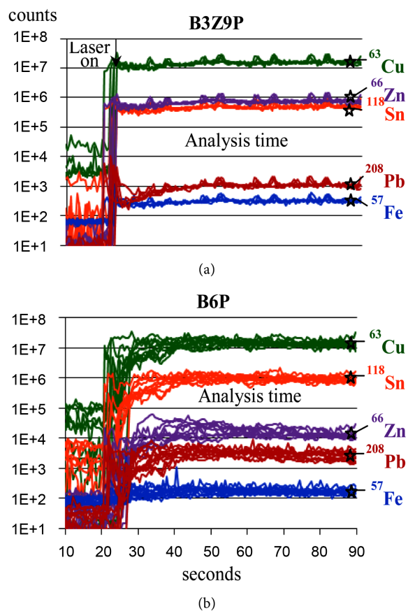
Figure 1. Typical NIR femtosecond LA-ICP-MS output from microanalysis of (a) B3Z9P and (b) B6P alloy reference materials.
