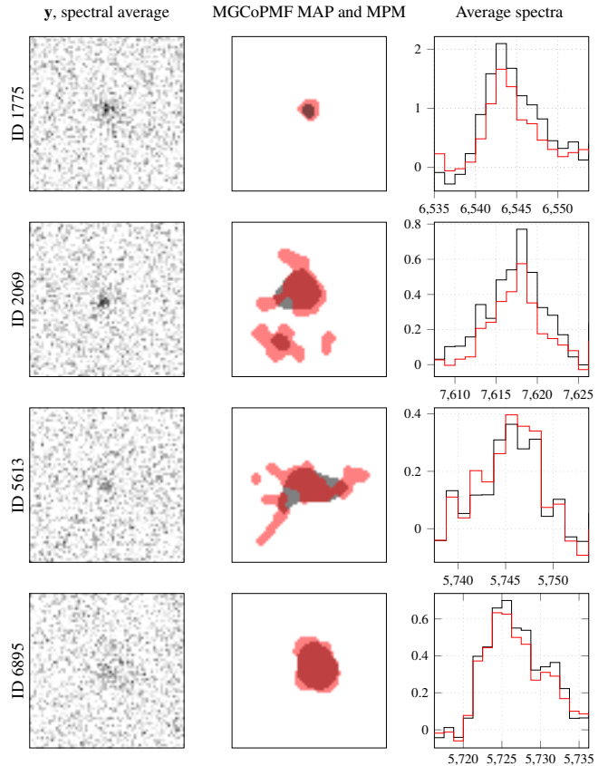
Figure 6: Results on 4 real MUSE images. Left : spectral average of \mathbf{Y} = \mathbf{y} (inverse video) after the spectral median subtraction has removed the brightest objects. Center : detection results with the MGCoPMF model, using the MPM (gray) and MAP (red) criteria. Right : average spectra in the two detected regions, with intensities in 10^{-20} \text{ erg s}^{-1} \text{ cm}^{-2} \text{ \AA}^{-1} as a function of the wavelength (in Ångström).
