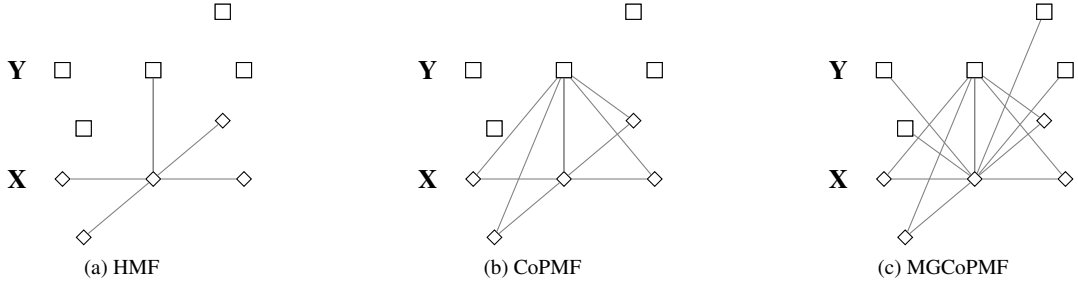
Figure 1: Dependency graph corresponding to the CoPMF models introduced in this paper. The graphs represent the distribution of (\mathbf{X}, \mathbf{Y}) given the center node (X_s, Y_s) . Roughly speaking, eliminating a graph edge is equivalent to not account for a variable in one of the conditional distributions ruling the process (\mathbf{X}, \mathbf{Y}) . The graph correspond to a local neighborhood, restricted to 4 sites for clarity purpose.
