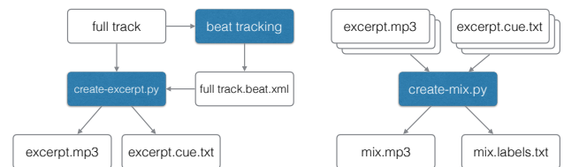
Figure 1. Data flow and file types of the UnmixDB dataset.
