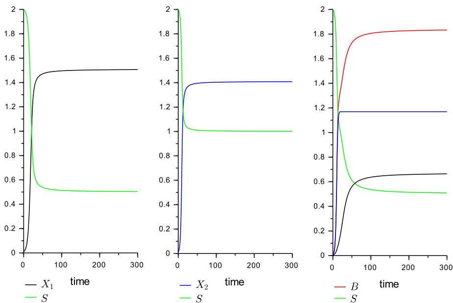
Fig. 3. From left to right: pure culture of species 1, pure culture of species 2 and mixed culture with both species.
