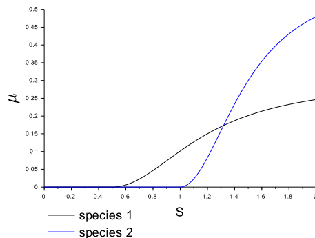
Fig. 2. Graphs of the two growth rate functions.
