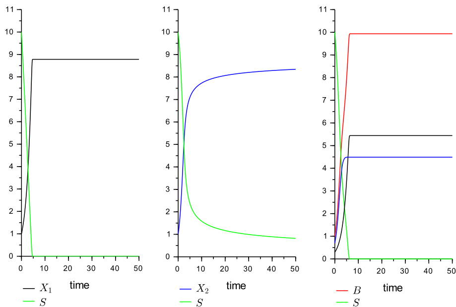
Fig. 5. From left to right: pure culture of species 1, pure culture of species 2 and mixed culture with both species.
