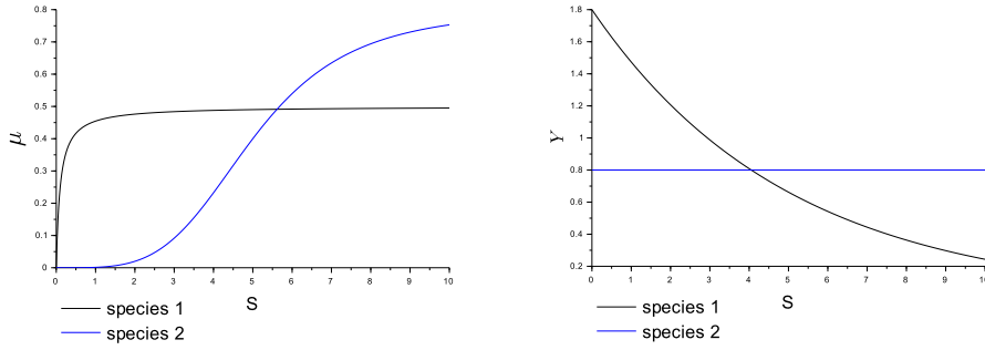
Fig. 4. Graphs of the growth rate functions (on the left) and yield functions (right).
