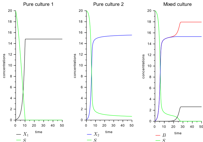
Fig. 7. From left to right: pure culture of species 1 ( X_1 ), pure culture of species 2 ( X_2 ) and mixed culture ( B = X_1 + X_2 ) with initial proportion X_1(0) = 10^{-4}B_0 . In green the concentration of substrate ( S ).
