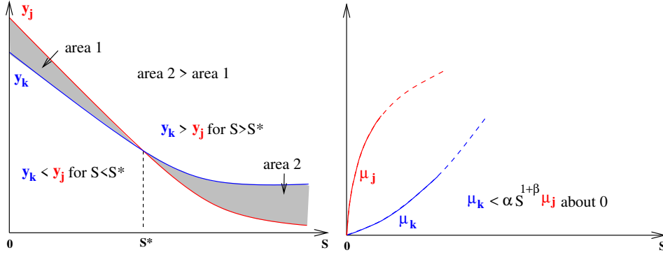
Fig. 1. Graphical illustration of sufficient conditions for overyielding.
