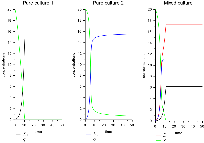
Fig. 6. From left to right: pure culture of species 1 ( X_1 ), pure culture of species 2 ( X_2 ) and mixed culture ( B = X_1 + X_2 ) with initial proportion X_1(0) = 0.3B_0 . In green the concentration of substrate ( S ).
