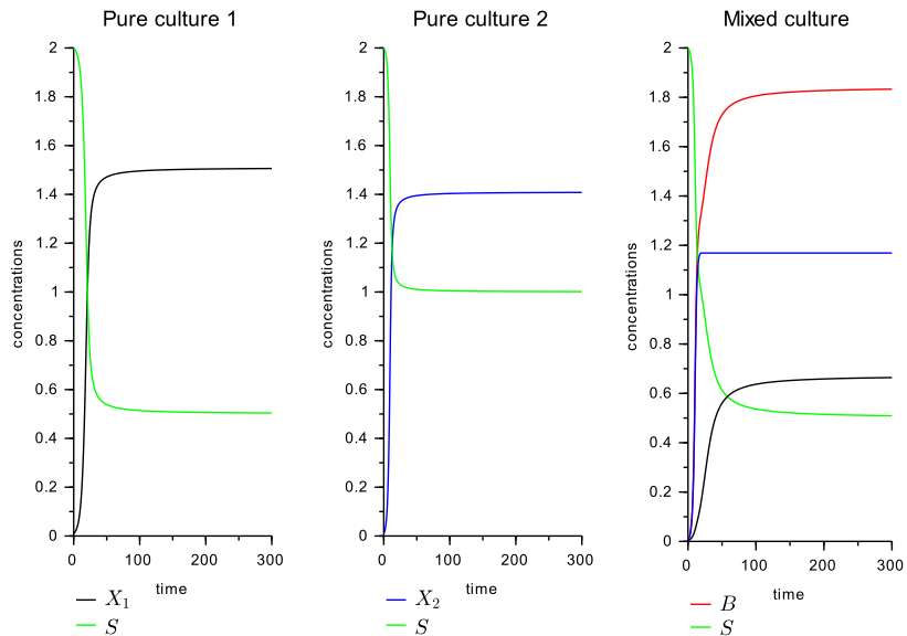
Fig. 4. From left to right: pure culture of species 1 ( X_1 ), pure culture of species 2 ( X_2 ) and mixed culture ( B = X_1 + X_2 ) with initial proportion X_1(0) = 0.4B(0) . In green the concentration of substrate ( S ).
