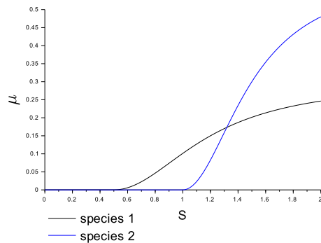
Fig. 3. Graphs of the growth rate functions given by expression (18) and parameters in Table 1.
