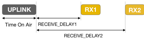
Fig. 1: Class A end-devices receive slot timing.
