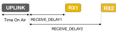
Fig. 1: Class A end-devices receive slot timing.
