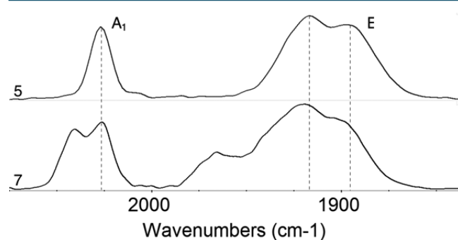
Figure 1. IR spectra obtained using ATR mode between 1820 and 2075 \text{cm}^{-1} of 5 in acetone and 7 in water (2 \text{mg}\cdot\text{mL}^{-1} ). See also Figure S4 and Table S2 for the spectra of 5 in a range of solvents.
