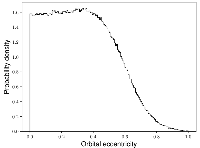
Fig. 7. Posterior probability of the orbital eccentricity of G196 b under the model including correlated noise.
