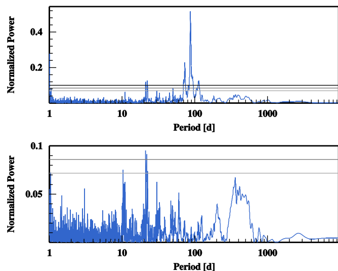
Fig. 19. Periodograms of: (top) the combined SOPHIE, CARMENES, and KECK radial velocities of Gl617A; (bottom) the residuals of a keplerian fit with P=86 d to the data. The horizontal lines correspond to 50%, 10%, and (top periodogram only) 1% FAP respectively.
