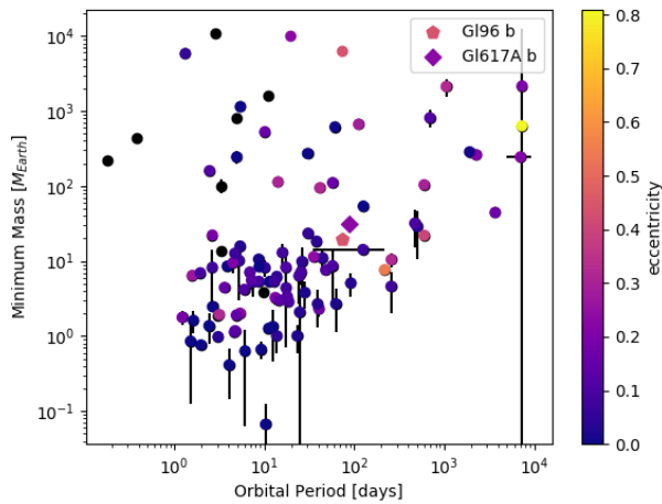
Fig. 23. Orbital period versus minimum mass for planets around M-dwarfs detected by radial velocities or transits. Each point represents a planet, with Gl96 b indicated by a pentagon and Gl617A b by a diamond. The colours indicate the orbital eccentricity.
