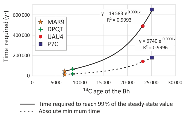
Figure 9. Relationship between the ^{14}\text{C} age of the Bh and the time needed to form the Bh (single-pool modelling).
