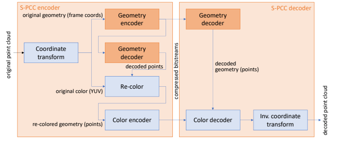
Fig. 8. Block diagram of the S-PCC encoder and decoder.
