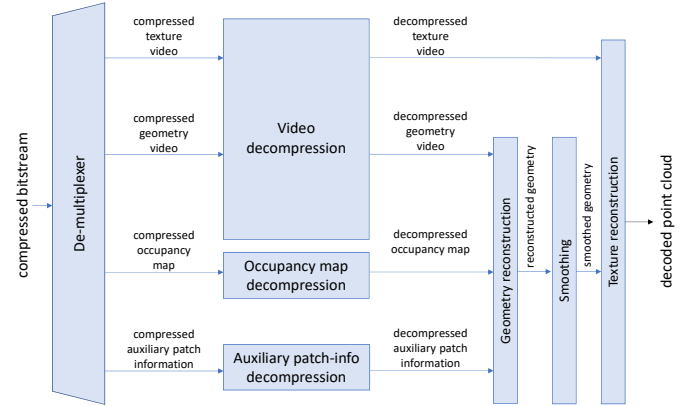
Fig. 12. Overview of the V-PCC decoding process.
