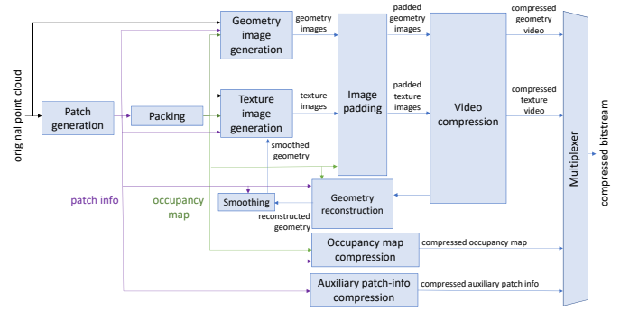
Fig. 11. Overview of the V-PCC encoding process.
