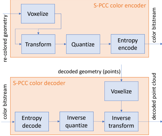
Fig. 10. Block diagram of S-PCC color encoder and decoder.
