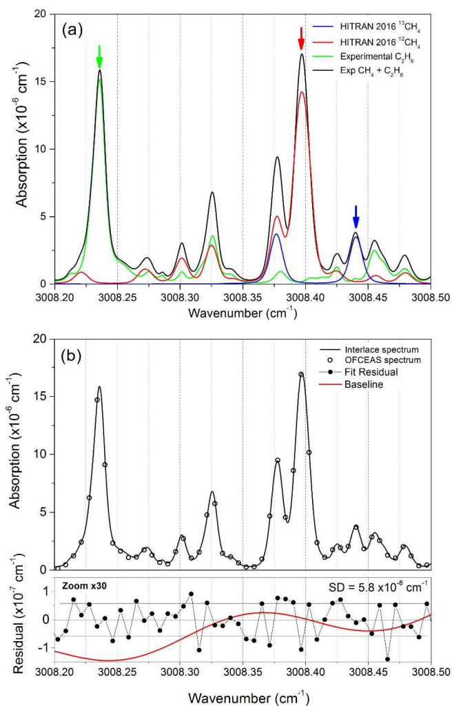
Figure 2 : (a) A combination of experimental interlaced spectra and spectra simulated using the HITRAN 2016 database at 30 mbar and 35°C. HITRAN profiles show the position of 12 CH 4 (red) and 13 CH 4 (blue) at 72 ppmv of CH 4 in dry air. In green, the interlaced spectrum acquired with only 20 ppmv of C 2 H 6 in dry air in the cavity. The full experimental spectrum containing absorptions from the three species is reported in black. There is a disagreement for the two superimposed lines at 3008.39 cm -1 , with a line intensity discrepancy between experimental data and the HITRAN 2016 database of ~16% on the amplitude of the absorption lines (this is outside the reported HITRAN 2016 uncertainties on the cross sections that are between 2% and 5%). (b) An example of an OFCEAS spectrum (black circles) and the corresponding interlaced methane-ethane absorption spectrum. At the bottom, the residuals of the spectral fit for one acquisition (0.1 s) and the baseline curve (red) are reported.
