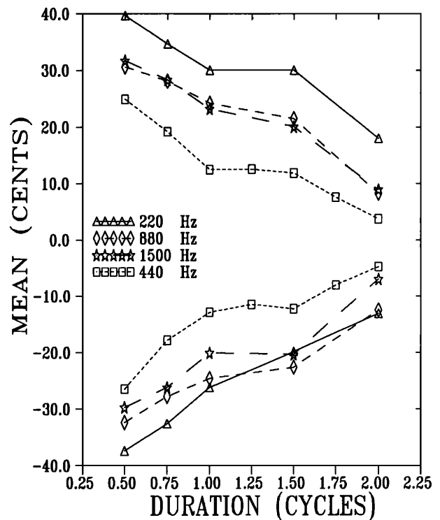
FIG. 9. Average settings for the parametric experiment on center frequency. X axis: pattern duration, in number of cycles. Y axis: difference between the mean pitch perceived and center frequency. Patterns sharing the same final phase are connected by a line. Vibrato extent: 100 cents, vibrato rate: 6 Hz.
