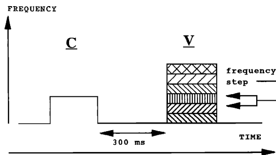
FIG. 2. Time line for the discrete-trial adjustment procedure: (V) vibrato tone, (C) varying constant- F_0 tone.
