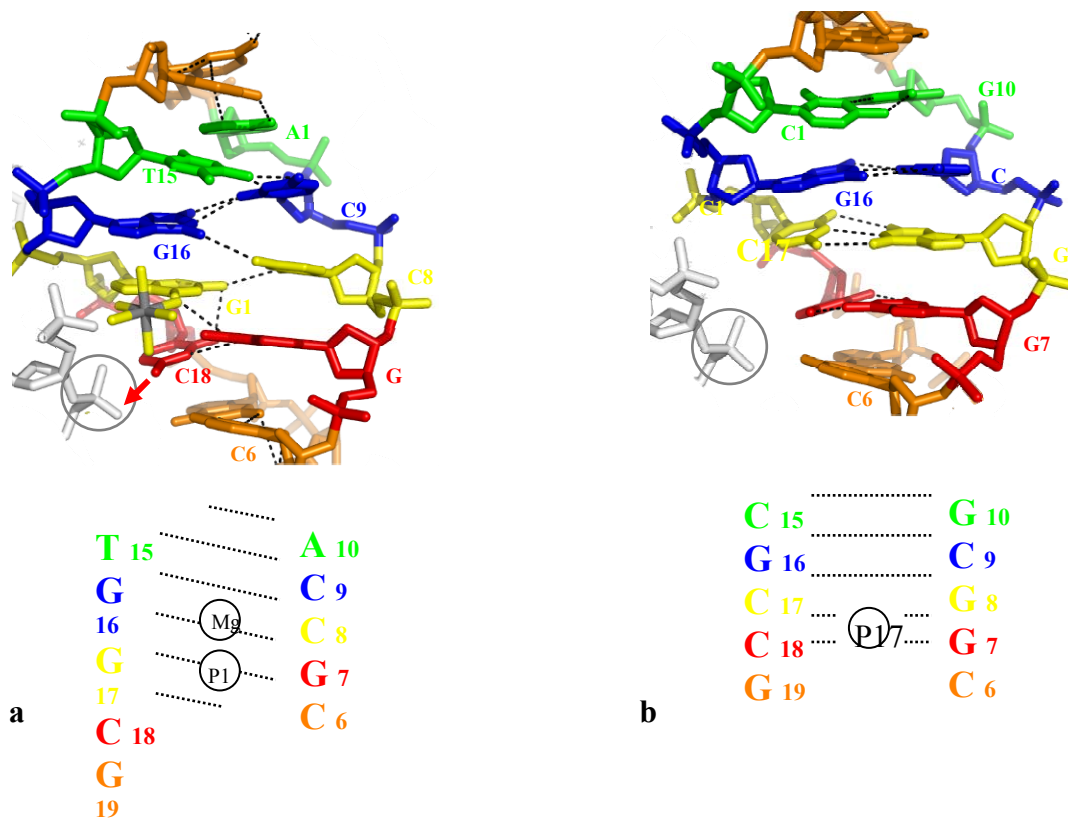
Figure 5. (a) Shift of the base pairing in the dodecamer d(ACCGGGCGCCACA). The backbone of the fitted molecule is represented in grey. The bases that should be normally paired are represented with the same color; (b) The corresponding region of the dodecamer d(ACCGCCGGCGCC) that displays a normal base pairing.
