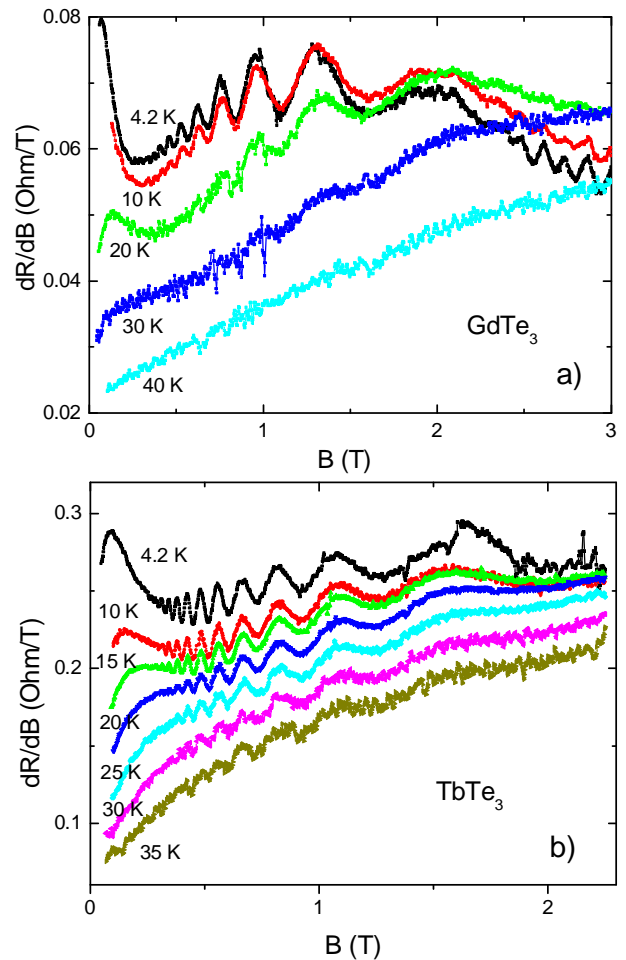
FIG. 3: (color online) Temperature evolution of slow oscillations in magnetoresistance for GdTe 3 (a) and TbTe 3 (b).
