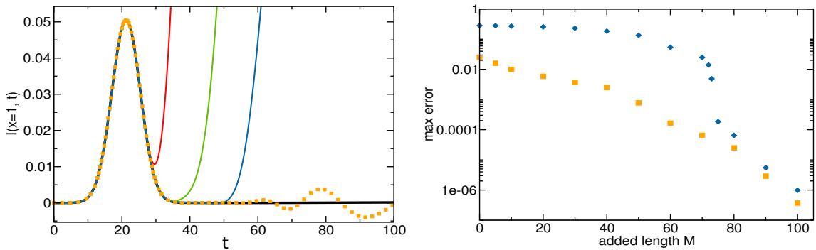
Figure 7: Comparative study of WF-B, C and D for N = 100 . E_F = -1\gamma and we send a Gaussian voltage pulse w(t) = V_P e^{-4 \log(2)t^2/\tau_P^2} with V_P = 0.05\gamma and \tau_P = 10\gamma^{-1} through the system. Left plot: current as a function of time just after the voltage drop for WF-B (black), WF-C with (from left to right) M = 10 (red), M = 20 (green), M = 30 (blue) and WF-D M = 30 (orange squares). Right graph: maximum error between t = 0\gamma^{-1} and t = 100\gamma^{-1} as a function of M for WF-C (blue diamonds) and WF-D (orange squares).
