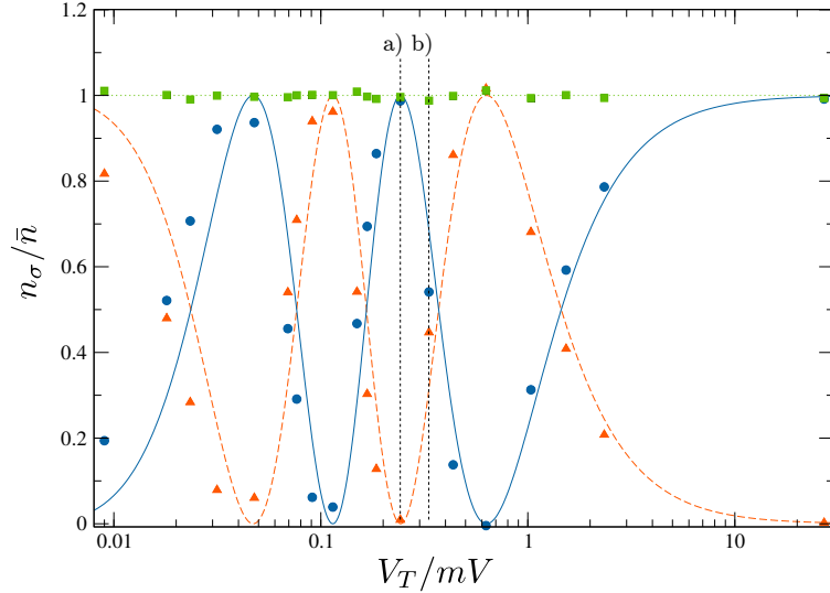
Figure 17: The number of transmitted particles through lead 2 (orange triangles) and lead 3 (blue circles) ( n_{\downarrow} and n_{\uparrow} , collectively n_{\sigma} ) normalized by the number of injected particles in lead 0 ( \bar{n} ) as a function of the tunneling gate potential, V_T . The green squares are the sum n_{\downarrow} + n_{\uparrow} . The corresponding lines are the DC transmission probabilities of the system between leads 0&2 (dashed orange) and 0&3 (full blue) and their sum (dotted green). The values of V_T indicated by the black dashed lines labeled a) and b) correspond to the values of V_T used to produce figure 18. These results were produced with a Gaussian voltage pulse as described in the main text.
