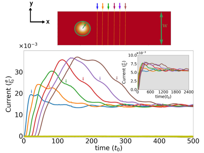
FIG. 2. Trace of the charge current computed at different interfaces in the waveguide. Each curve corresponds to the current probed at a specific interface, as indicated in the top sketch (dashed vertical lines). The colored arrows indicate the time when the skyrmion center crosses a specific interface. These interfaces are spaced by a distance of 10a and the parameters are W = 51a , 2R = 15a , v = 0.2a/t_0 , and \Delta = 0.1\gamma . The yellow downward triangles denote the current pumped by a 1D DW with the same parameters. The inset is obtained for v = 0.05a/t_0 .
