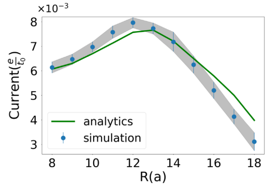
FIG. 3. Stationary current pumped by one skyrmion as a function of its radius as computed numerically (blue symbols) and analytically (green solid line). The gray region is the range of the fluctuation due to lattice effects (i.e., the ripples in Fig. 2). The velocity is v = 0.07a/t_0 and the other parameters are the same as in Fig. 1.
