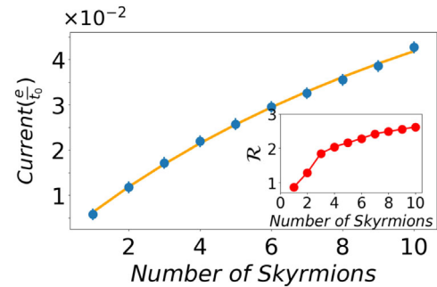
FIG. 4. Pumped current as a function of the number of skyrmions. The blue dots represent the current computed numerically and the orange line is the fit with the equation for N skyrmions given in the main text. The inset displays the reflection coefficient as a function of the number of skyrmions. The parameters are W = 31a , \Delta = 0.1\gamma , v = 0.15a/t_0 , R = 7.5a , E_F = -3.5\gamma .
