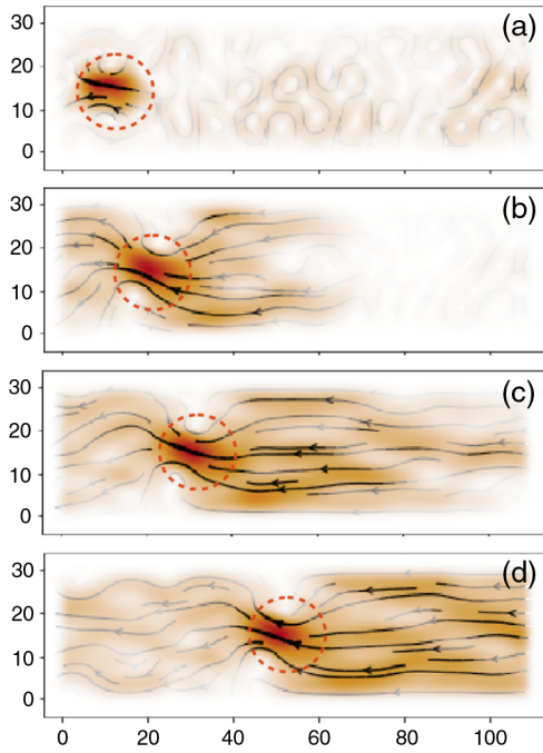
FIG. 1. 2D map of the current lines at different times. (a) t = 4t_0 , (b) 50t_0 , (c) 100t_0 , and (d) 200t_0 . The black arrows denote the direction of the charge current, and the color shading denotes amounts for the current gradient. The dark shaded region reveals the position of the skyrmion, where the current gradient is maximum. The parameters are v = 0.2a/t_0 , W = 31a , 2R = 15a , and E_F = -3.8\gamma . Initial skyrmion position is x(0) = 15a .
