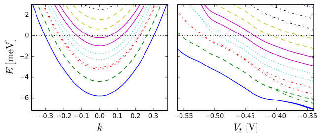
FIG. 7. (Color online) Structure of the subbands in the central region. Left panel: Energy dispersion E(k) versus k for V_t = -0.43 \text{ V} . The bands that cross the Fermi energy E = E_F = 0 correspond to propagating channels. Right panel: Transverse energies E(k = 0) of the different modes as a function of the tunneling voltage V_t . The bands below the Fermi energy are propagating. Parameters: V_m = -0.495 \text{ V} and V_l = -0.45 \text{ V} for both panels. Symmetric/Antisymmetric modes pairs are plotted with similar color and line style.
