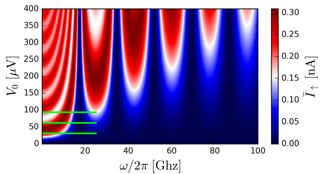
FIG. 2. (Color online) Rectified DC current from Eq. (9a) for \delta_F = 0.32\pi and \tau = 58 ps. The results of Fig. 4 correspond to cuts along the green lines.
