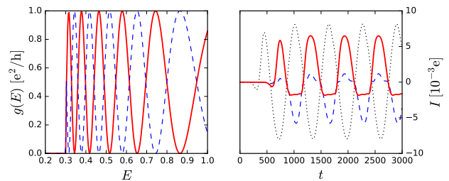
FIG. 3. (Color online) Simple microscopic model. Left panel: DC differential conductances g_{\uparrow\uparrow}(E) (dashed blue line) and g_{\downarrow\uparrow}(E) (straight red line) as obtained from a direct numerical calculation of the tight-binding model. The numerical calculations were performed with the Kwant 33 package. The reflection probability from L\uparrow to L\uparrow or L\downarrow vanishes in the region of interest. Right panel: currents in R\downarrow (straight red line, I_{\downarrow}(t) ) and R\uparrow (dashed blue line, I_{\uparrow}(t) ) after a microwave excitation in L\uparrow (dotted black line) computed using time dependent simulations of the microscopic model.
