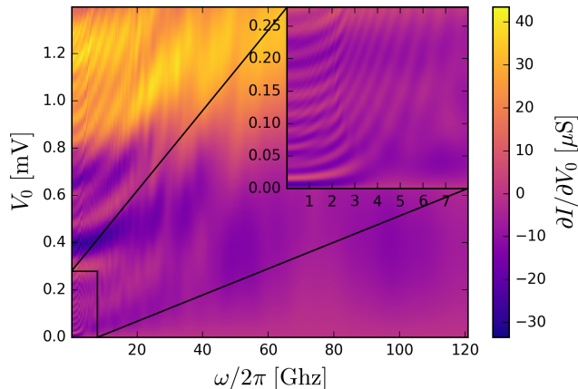
FIG. 10. (Color online) Realistic microscopic model. Colormap of \partial\bar{I}_\uparrow/\partial V_0 - \partial\bar{I}_\downarrow/\partial V_0 versus voltage amplitude V_0 and frequency \omega/2\pi . The inset shows a zoom of the main panel. Two channels with \tau = 220 ps (oscillations visible in the inset) and \tau = 19 ps (oscillations visible in the main panel) dominate the signal. Calculations performed at 20 mK.
