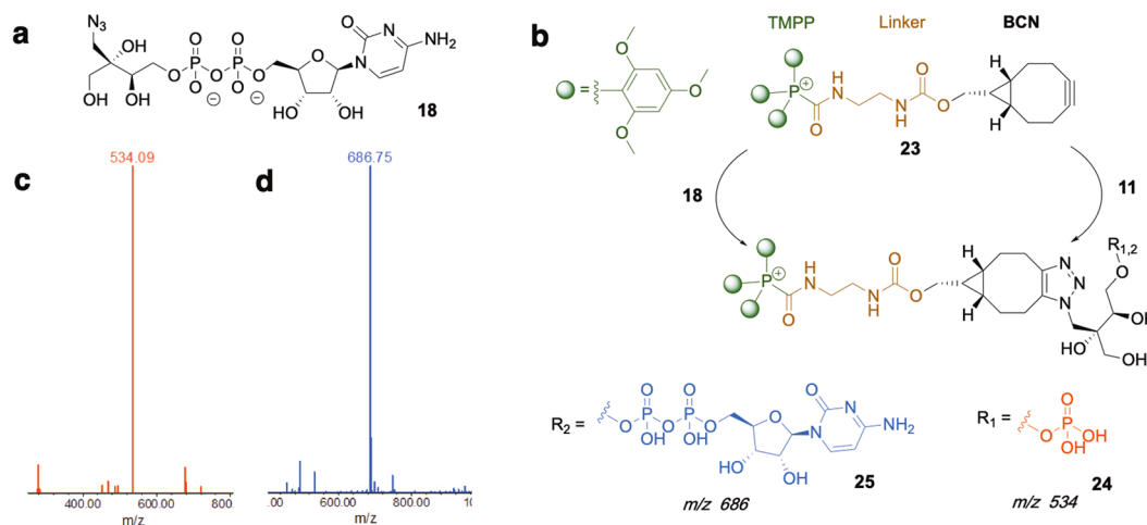
Figure 3. LC-MS analysis of MEPN 3 or its product in the YgbP catalysed reaction after derivatisation with TMPP-BCN ( 23 ). (a) Structure of CDP-MEN 3 , (b) Structure of MEPN 3 or of its product after derivatisation with TMPP-BCN. (c) Mass-to-charge ratio of MEPN 3 clicked with TMPP-BCN. (d) Mass-to-charge ratio of the product of 11 in the YgbP catalysed reaction clicked with 23 .
