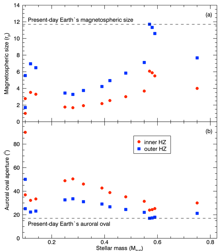
Fig. 2. (a) Upper limit of magnetospheric sizes and (b) the corresponding apertures of their auroral ovals for hypothetical planets orbiting the dM stars in our sample. We assume that these planets harbour dipolar magnetic fields with the same intensity as that of the Earth. For comparison, the dashed line shows the present-day Earth's magnetospheric size (upper panel) and the Earth's auroral oval aperture (lower panel).
