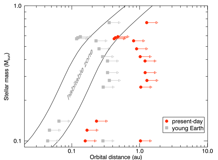
Fig. 3. Closest orbital distance at which an Earth-like planet orbiting the stars in our sample would be able to sustain the present-day (red circles) and the young (3.4 Gyr ago, grey squares) Earth’s magnetospheric size, assuming it has the same magnetic field as the Earth. We use a sample of 15 active stars for which large-scale surface magnetic-field maps were reconstructed, to determine the magnetic pressure at the planet orbit and hence the largest extent of its magnetosphere. Planets orbiting at a closer orbital radius would experience a stronger stellar magnetic pressure, which could reduce the size of the planet’s magnetosphere significantly, exposing the planet’s atmosphere to erosion by the stellar wind. For reference, we show the inner/outer edge of the HZ for 1-Gyr-old low-mass stars (solid lines).
