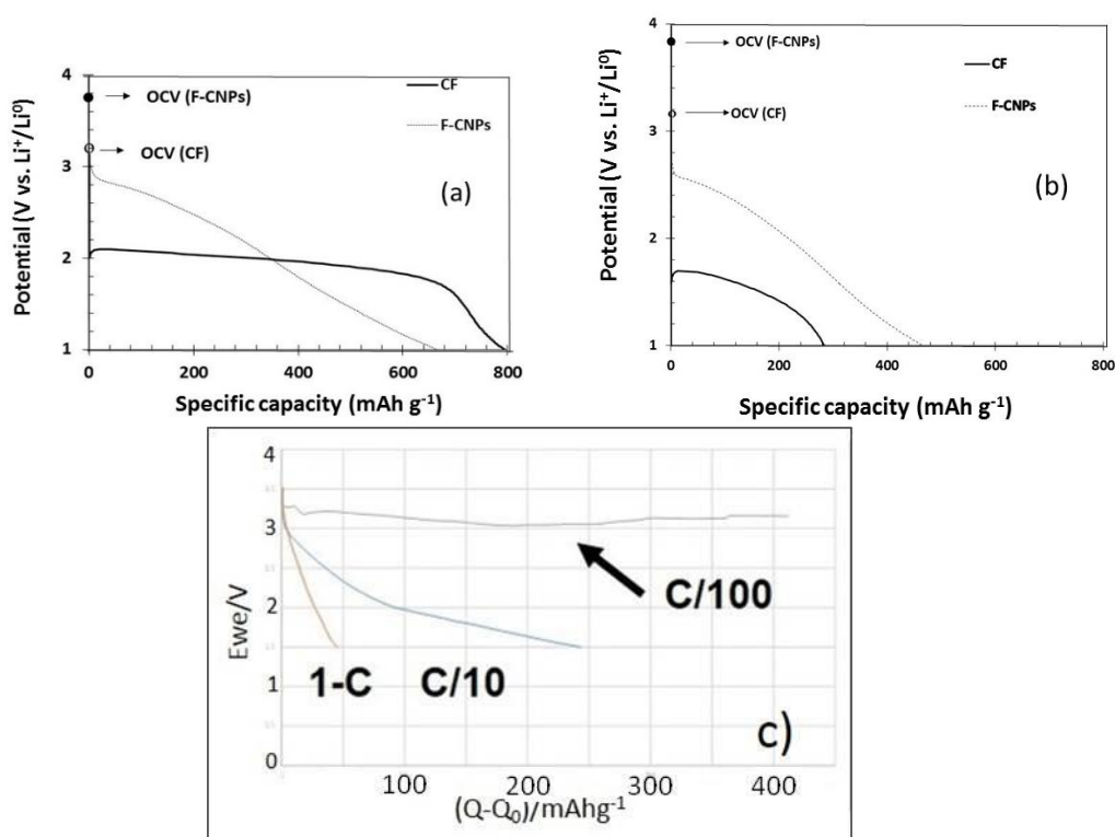
Fig. 10. Comparison of the discharge curves obtained with commercial CF x (CF ~0.65 ) and F-CNP (CF ~0.43 ) at a) C/5 rate and b) 1C rate. Discharge curves of F-CNPs-based Li-battery at c) 1C, C/10, and C/100 rates.
