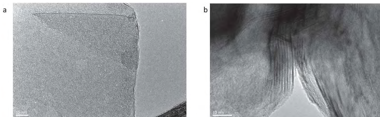
Supplementary Figure 5 | TEM micrographs of hollow Ti 3 C 2 spheres. a, edge of an individual Ti 3 C 2 T x flake, confirming presence of single-layer flakes and b, the connection point of two Ti 3 C 2 T x hollow spheres. They are with few layers and share some of them, indicating a good connection. This is important for the charge transfer throughout the entire macroporous framework.
