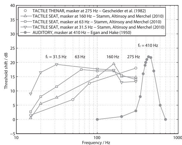
Figure 5: Auditory and vibrotactile masked thresholds relative to un-masked condition as a function of frequency. The vibration maskers were narrow band noises centered at 31.5 Hz, 63 Hz, 160 Hz and 275 Hz with fixed level approximately 25 dB above threshold. Data from Stamm, Altinsoy and Merchel [47] are plotted for whole-body vibrations (25 Hz noise bandwidth) and from Gescheider et al. [21] for vibrations at the thenar eminence (100 Hz noise bandwidth). For comparison, an auditory masking pattern is plotted for a 90 Hz wide band of masking noise, centered at 410 Hz with 40 dB SPL [6]. Test stimuli were simultaneously presented sinusoids in all conditions.
