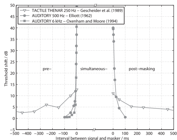
Figure 6: Auditory and vibrotactile pre- and post-masking as a function of the gap between signal and masker. Data from Gescheider et al. [17] is plotted using a 250 Hz vibration masker at the thenar eminence with 20 dB sensation level. The test signal was also a 250 Hz vibration. For comparison, auditory data from Elliott [9] is plotted using a white noise masker at 90 dB SPL. The test signal was a tone at 500 Hz. Additionally, pre-masking is plotted after Oxenham and Moore [43] using a noise masker and a 6 kHz tone.
