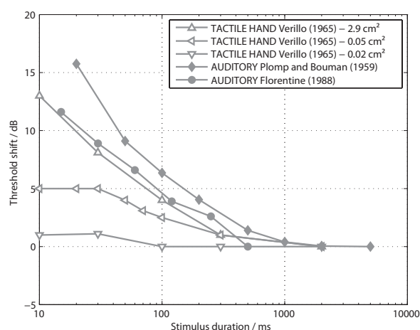
Figure 4: Auditory and vibrotactile threshold shift as a function of burst duration after [44, 12, 51]. Data are plotted in dB re threshold of detection for the longest stimulus of each curve. In all cases, the stimuli frequency was 250 Hz. The vibrotactile stimuli were applied to the skin of the hand using different contactor sizes.
