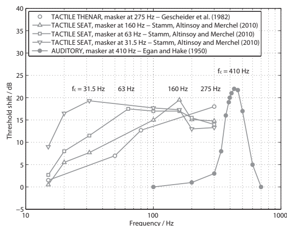
Figure 5: Auditory and vibrotactile masked thresholds relative to unmasked condition as a function of frequency. The vibration masker were narrow band noises centered at 31.5 Hz, 63 Hz, 160 Hz and 275 Hz with fixed level approximately 25 dB above threshold. Data from Stamm, Altinsoy and Merchel [47] are plotted for whole-body vibrations (25 Hz noise bandwidth) and from Gescheider et al. [21] for vibrations at the thenar eminence (100 Hz noise bandwidth). For comparison, an auditory masking pattern is plotted for a 90 Hz wide band of masking noise, centered at 410 Hz with 40 dB SPL [6]. Test stimuli were simultaneously presented sinusoids in all conditions.
