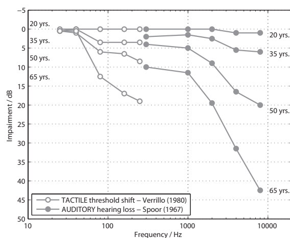
Figure 3: Auditory and vibrotactile threshold shift as a function of age. Auditory data depicts presbycusis (without the effects of severe occupational noise) [46]. Vibrotactile data are achieved using a 2.9 \text{ cm}^2 contactor at the thenar eminence [56] and plotted relative to the threshold at 20 years. The data points at 250 Hz are shifted slightly for better illustration.
