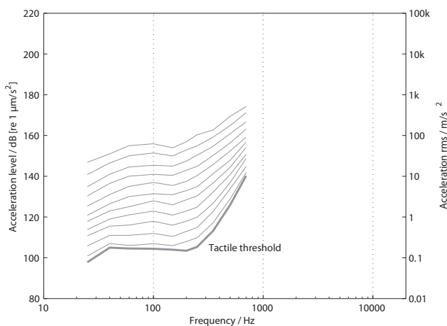
Figure 2: Curves of equal subjective intensity plotted as a function of frequency for vibrations of a 2.9 \text{ cm}^2 contactor on the thenar eminence (adapted from Verrillo [59]).
