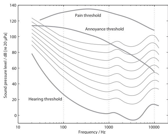
Figure 1: Curves of equal subjective intensity plotted as a function of frequency for sounds (according to ISO 226:2003 [29] and Winckel [64]).
