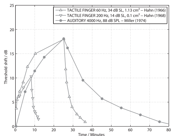
Figure 7: Auditory and vibrotactile temporary threshold shifts during and after exposure to long-lasting stimulation. Data from Hahn [25, 26] is plotted for vibratory stimulation of the Pacinian channel with different intensities and durations. For comparison, an exemplary temporary threshold shift for the auditory system is plotted after Miller [39].
