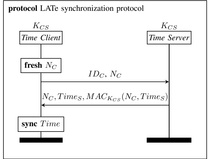
Fig. 1. LAtE Synchronization Protocol Diagram. K_{CS} is a symmetric pre-shared key between the Time Client (TC) and the Time Server (TS) . ID_C is the identity representation of TC . N_C is a nonce generated by TC .
