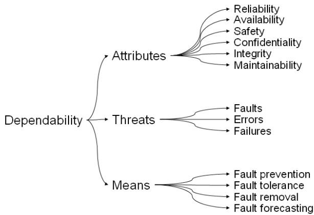
Fig. 2 - Dependability tree following Laprie et al.
