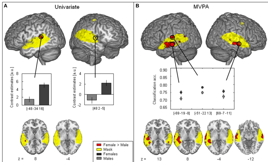
FIGURE 2 | Contrast between female > male (red). (A) Univariate analysis showing significant female > male difference (two-sample t -test, FWE-corrected, p < 0.05 ) in the left posterior part of the superior temporal gyrus (STG) and the right anterior STG. Contrast estimates at peak voxel showing stronger activation in females (black) as compared to males (gray) in response to vocal vs. non-vocal sounds. (B) MVPA showing significant classification accuracy above chance level in the right middle part of the
