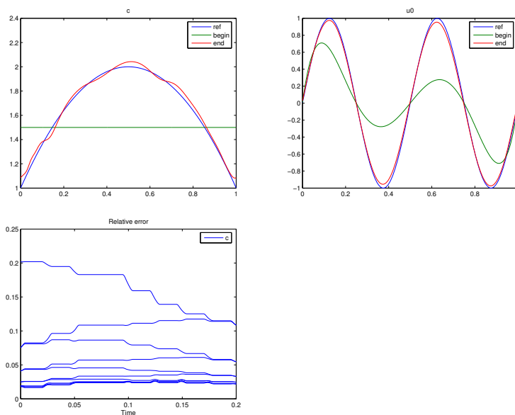
Fig. 1 Comparisons between the true augmented state (state and parameter) and its estimation by P-BFN algorithm: reconstruction of parameter (left) and state (right). Relative error of parameter reconstruction (bottom) with regards to P-BFN iterations in a time window of [0, T] equal to [0, 0.2] .
