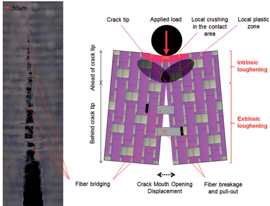
Figure 12. Illustration of crack extension and crack mouth opening displacement in SENB specimens at 150°C ( a/w = 0.3 ): influence of fiber bridging on extrinsic toughness. SENB: single edge notch bending.
